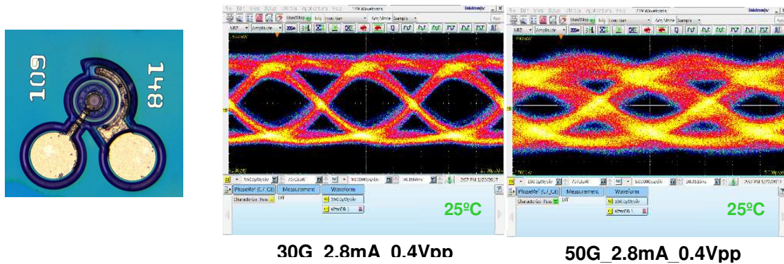
Figure 2: VCSEL chip micrograph and large signal performance at 30 Gb/s and 50 Gb/s.
