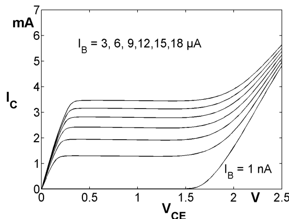
Fig. 4: Output characteristic of HBT with A_E = 0.13 \times 2.7 \mu\text{m}^2
