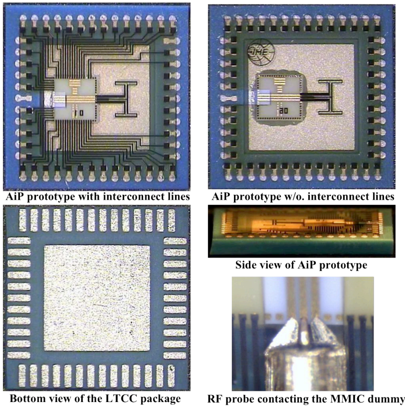
Figure 13 Antenna-in-Package Prototype
