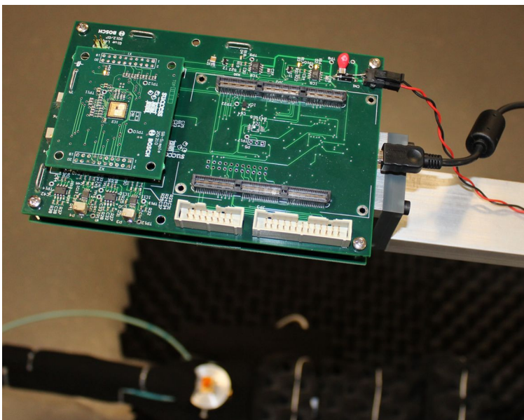
Figure 9 PCB in the measurement setup, and a detail view of the soldered sensor
