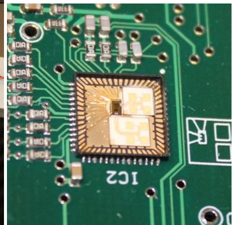
Figure 9 PCB in the measurement setup, and a detail view of the soldered sensor
