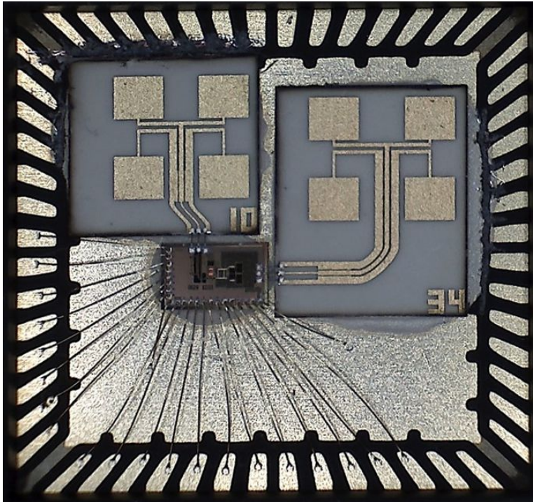
Figure 8 8 mm × 8 mm QFN package with integrated 122 GHz IC, transmit antenna (left), and receive antenna (right).
