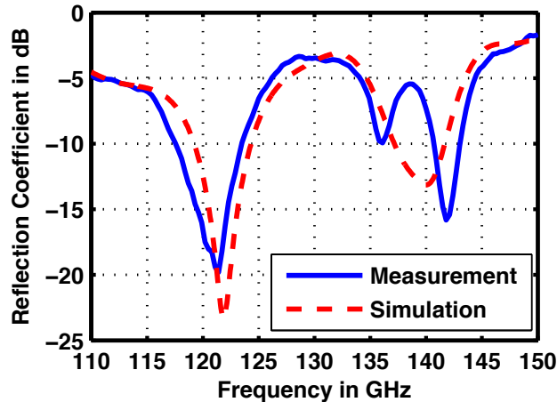
Figure 6 Simulated and measured reflection coefficient of the integrated antenna including the wire bond interconnect
