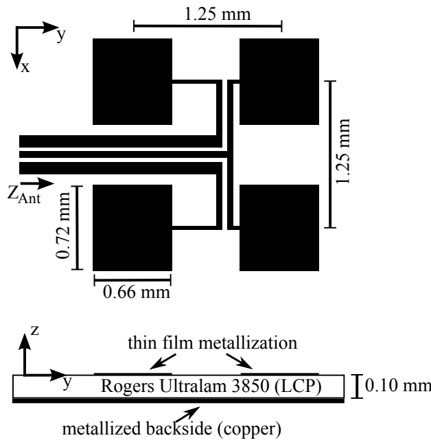
Figure 2 Antenna array with GCPW-feeding on 0.1 mm thick Rogers Ultralam 3850
