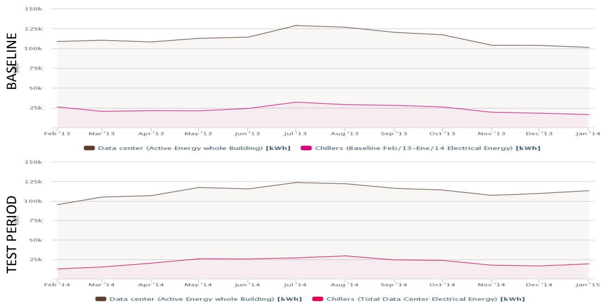
Data centre cooling optimization: Baseline vs Test period data
