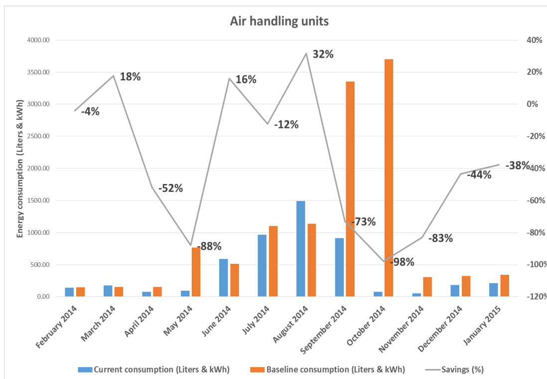
Air handling units: Baseline vs Test period data
