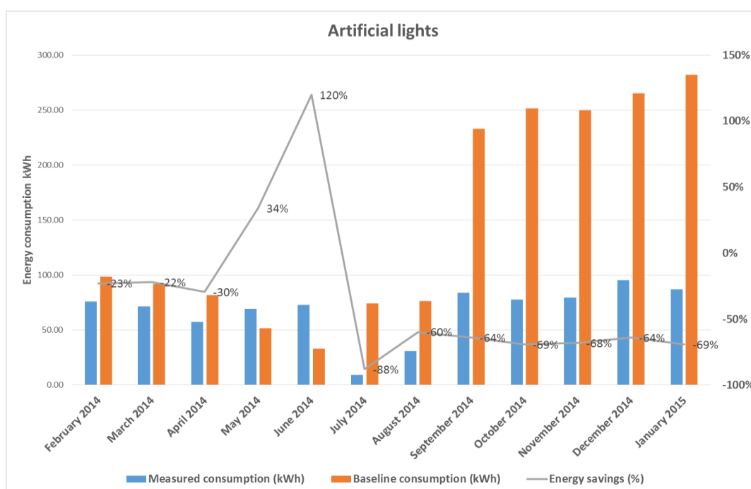
Artificial lights: Baseline vs Test period data
