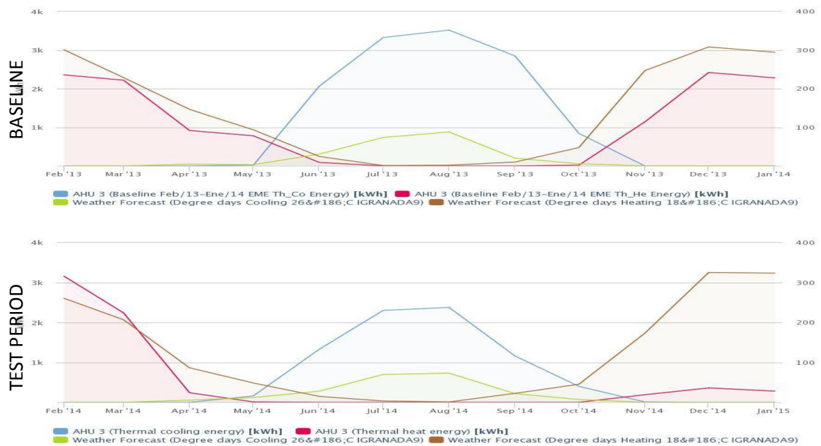
Emergency area AHU: Baseline vs Test period data
