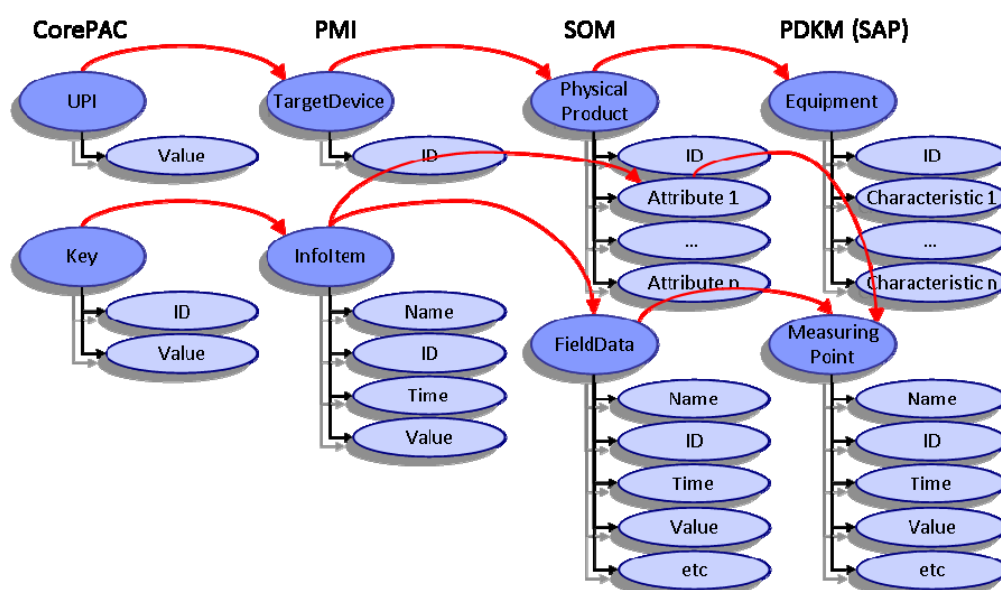
Figure 17: Mapping of CorePAC, PMI, SOM and PDKM classes and attributes
