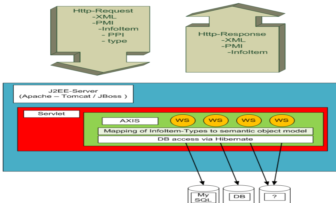
Figure 6: Concrete J2EE implementation of a PD(K)M
