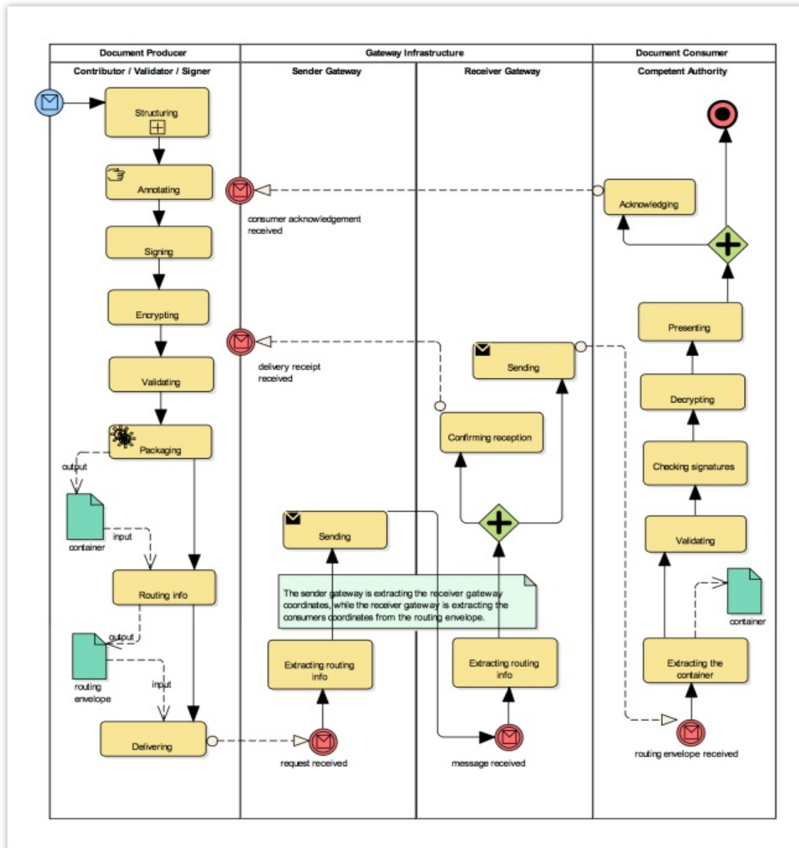
Figure 14. eDocument Architecture
