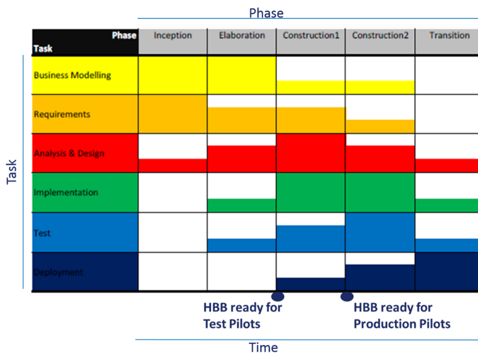
Figure 1: Unified Process
