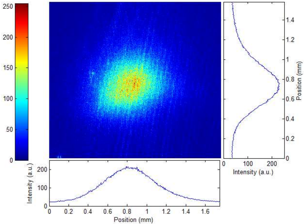
Fig. 3: Fluorescence image of a ^{87}\text{Rb} cloud of atoms in the MOT. Color coded is the light intensity collected by the CCD camera
