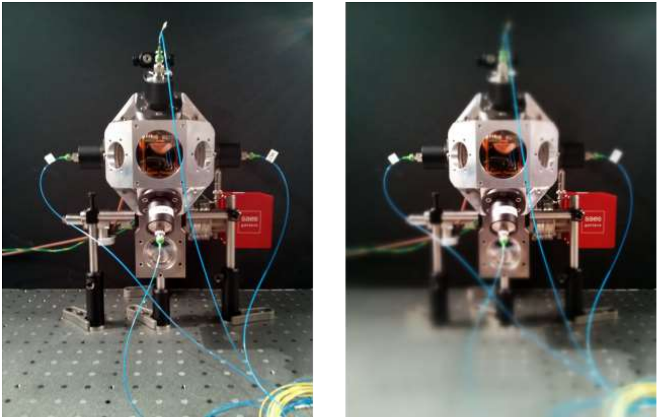
Fig 2: Science chamber setup with MOT fibres and telescopes
