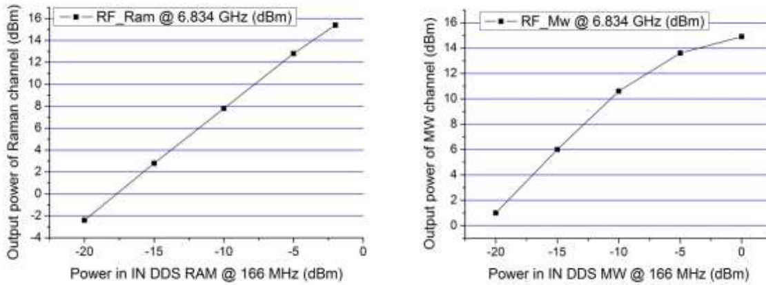
Fig. 3.2 - Output levels on the Raman and MW channels as a function of the DDS input power
