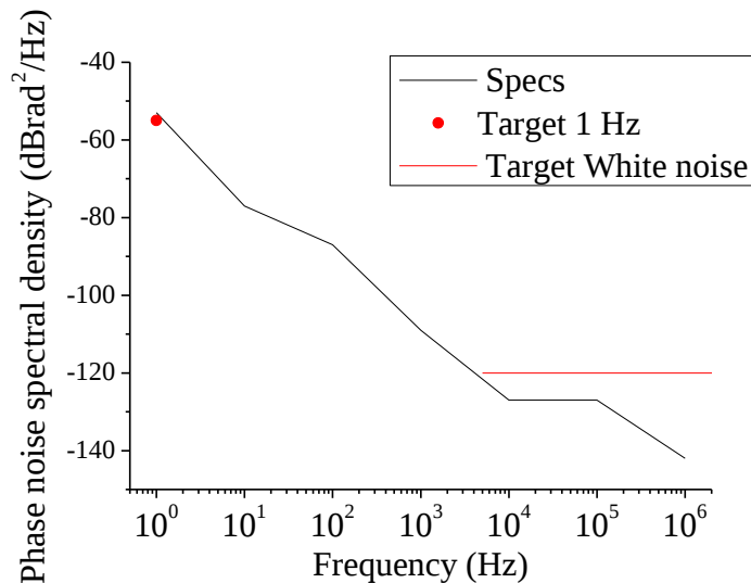
Fig. 3.3 - Phase noise power spectral density at 7 GHz (from the manufacturer specifications), and target specifications at 1 Hz and above 5 kHz.
