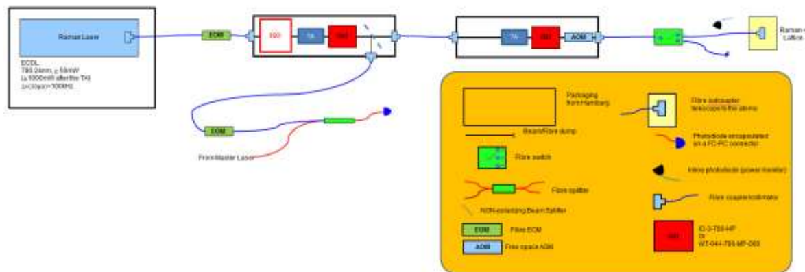
Fig. 4: Schematic of the Raman/Lattice laser
