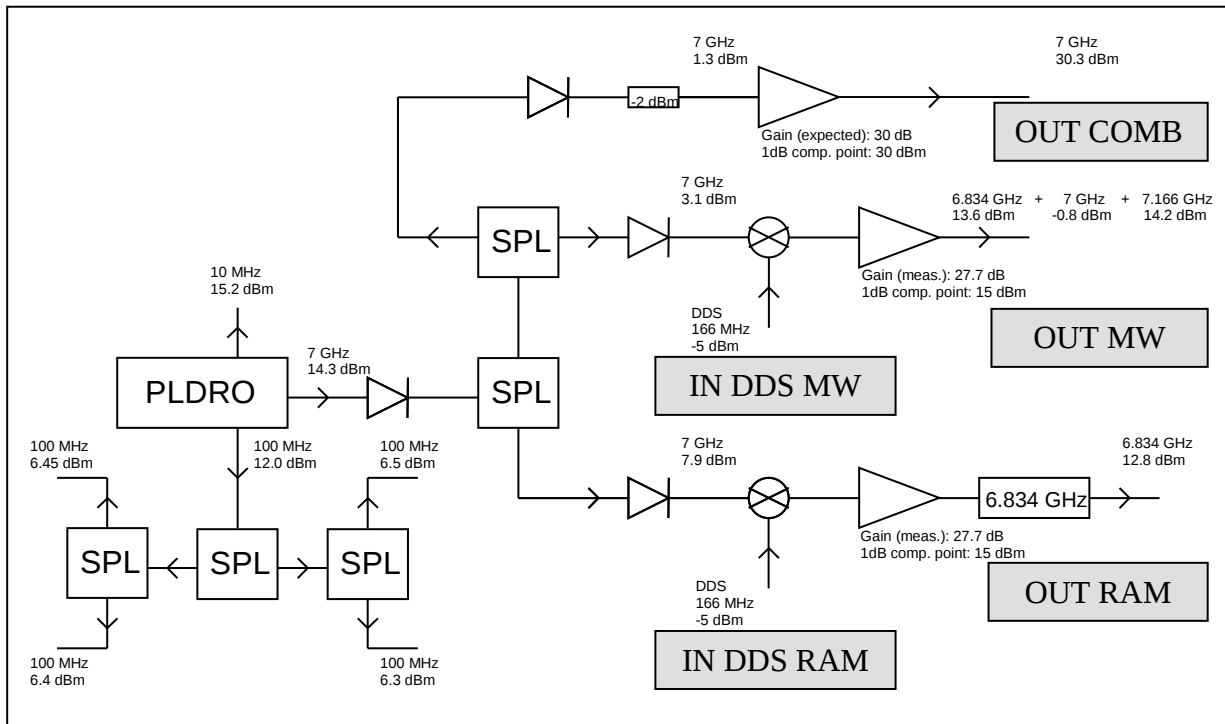
Fig.1 - Schematics of the PLDRO microwave chain
