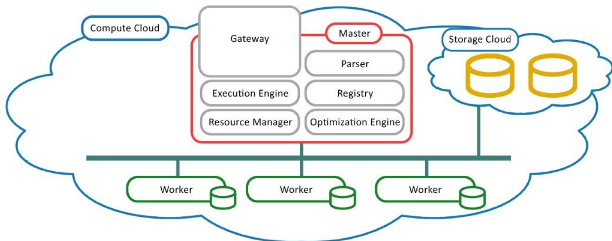
Figure 13: EXAREME's Architecture.
