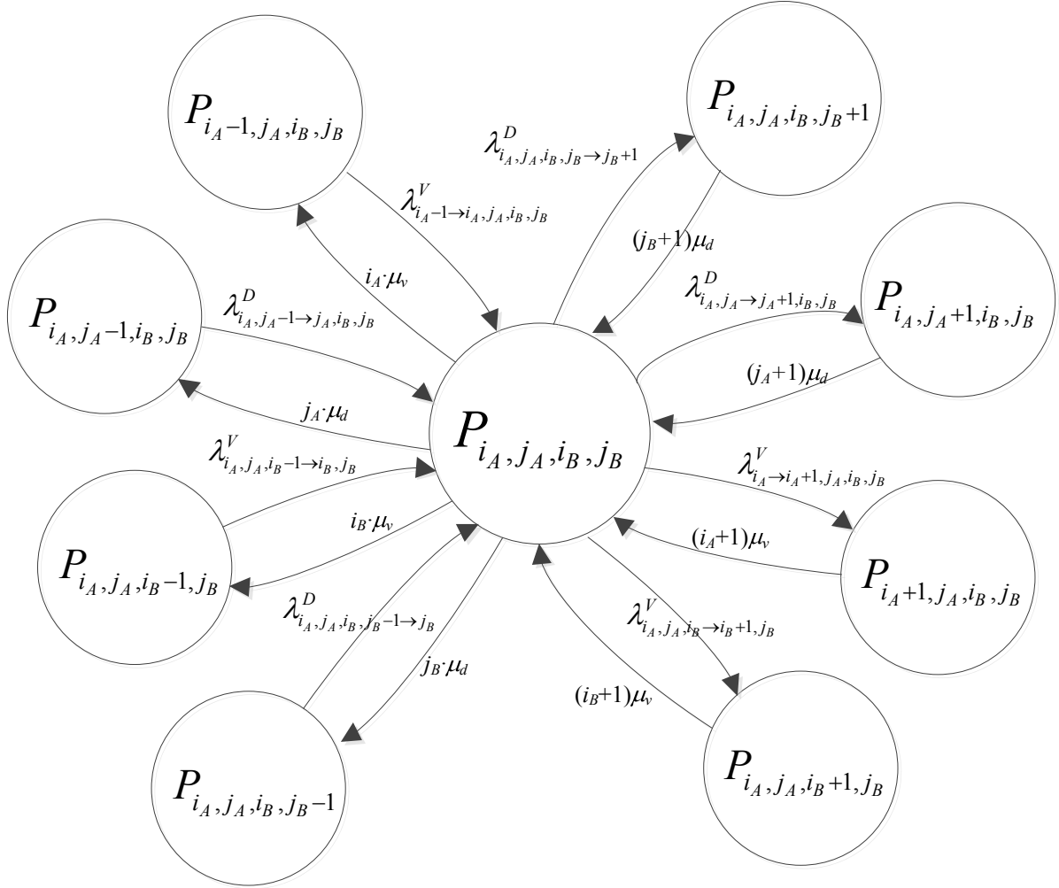
Figure 25. Links among the states of a 4D Markov chain characterising mixed voice and data users served by two colocated HNB with omnidirectional antennas
