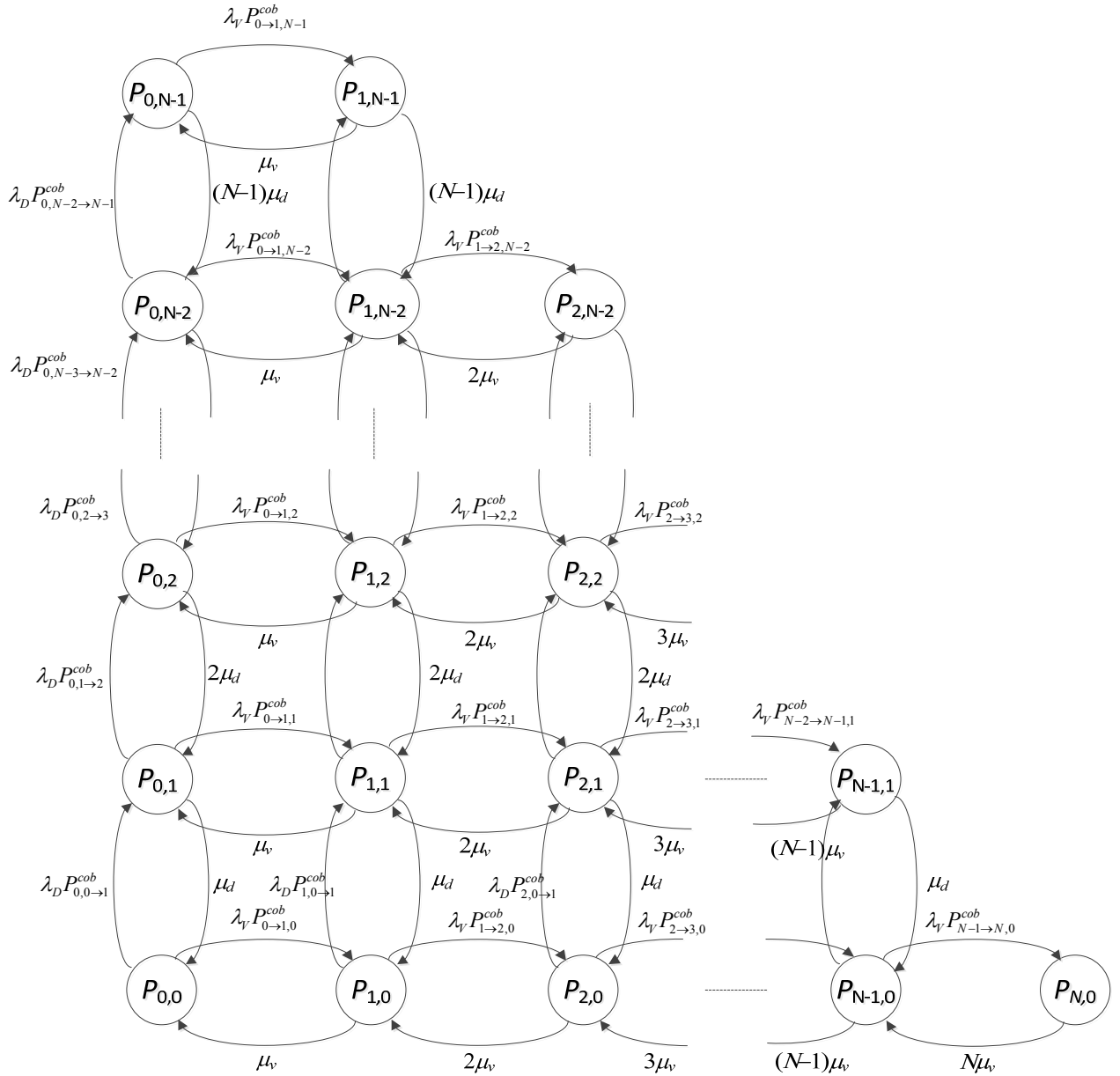
Figure 23. Markov chain characterising mixed voice and data users served by a HNB of N circuits, assuming a large number of subscribers
