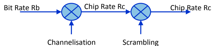
Figure 73. Combined use of the channelization and scrambling codes.
