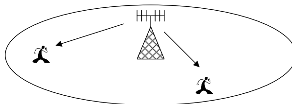
Figure 37. Intracell/noise-limited scenario
