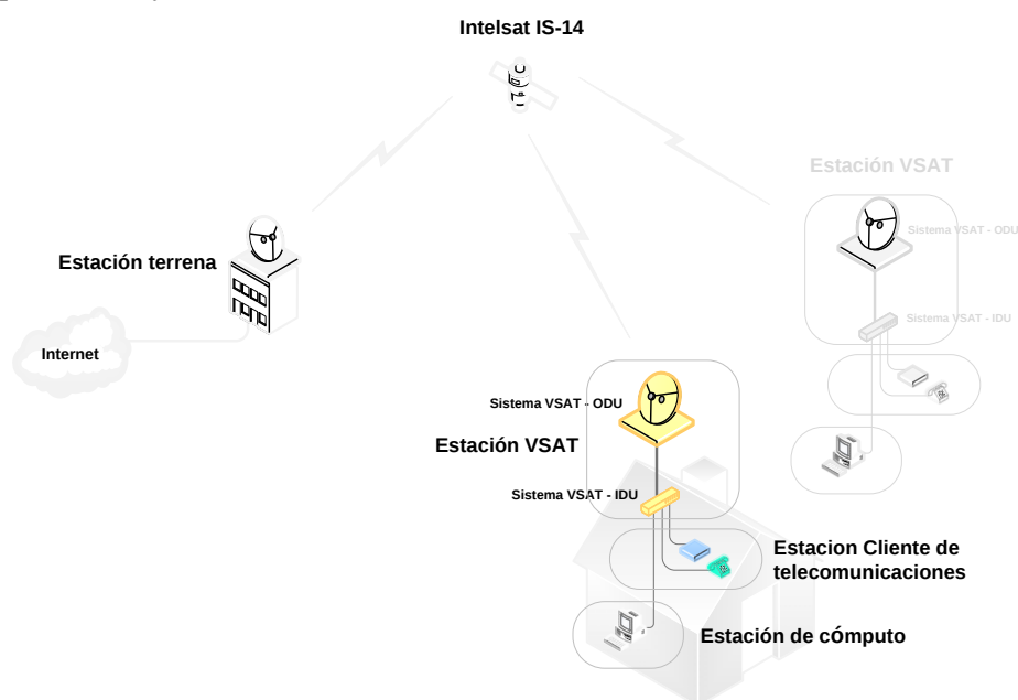
Figure 50. Scheme of a VSAT station
