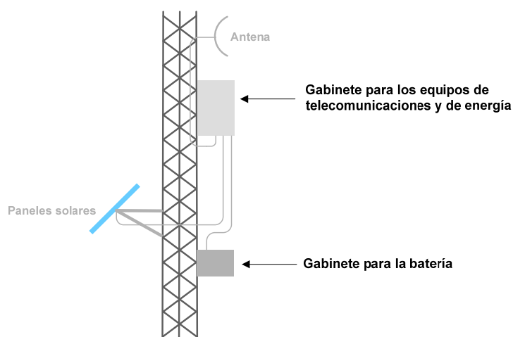
Figure 30. Cabinets on the Tower.
