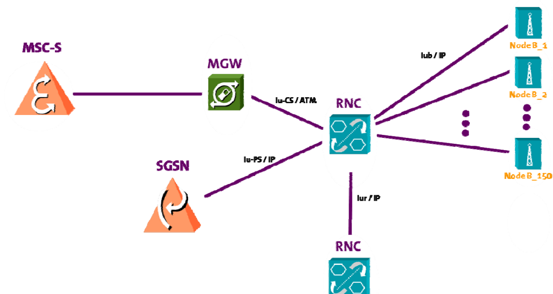
Figure 45. Femto controller connection diagram.
