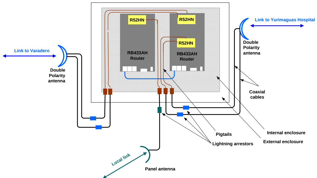
Figure 9: Diagram of the equipment in the San Juan node.
