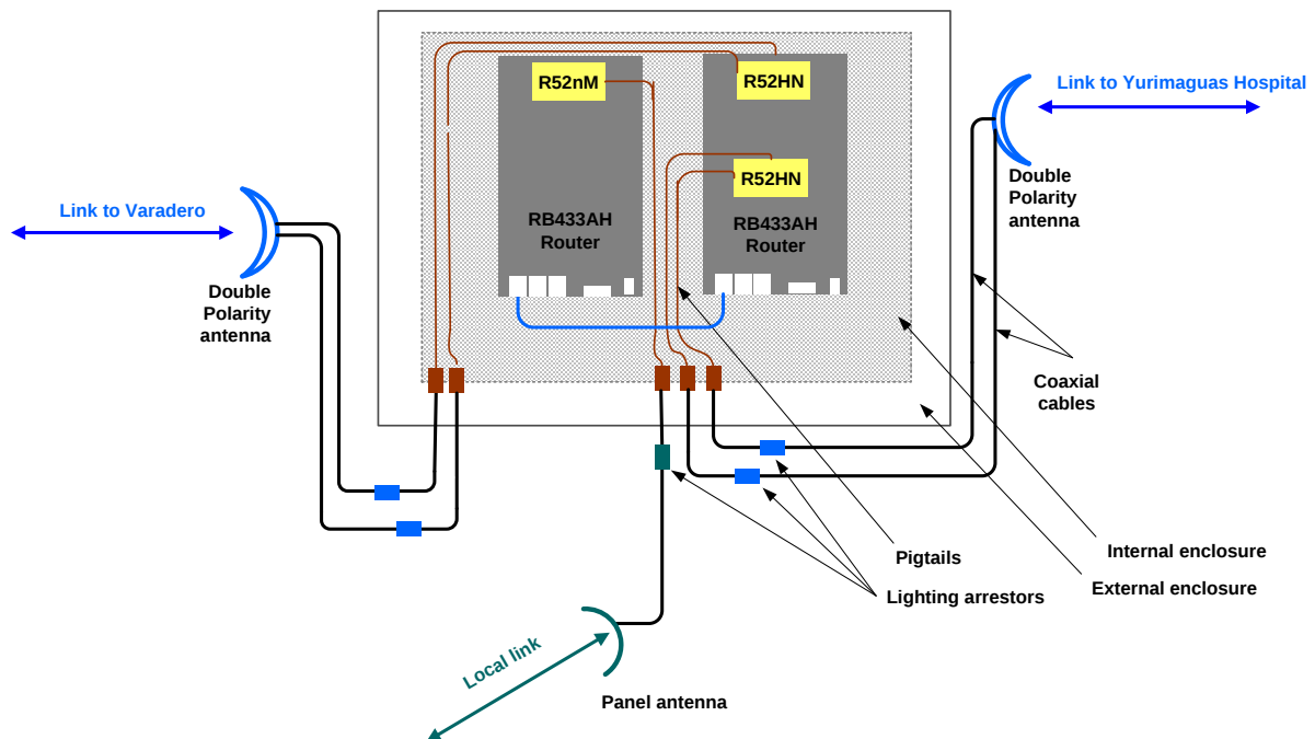
Figure 44: Diagram of the equipment in the San Juan repeater
