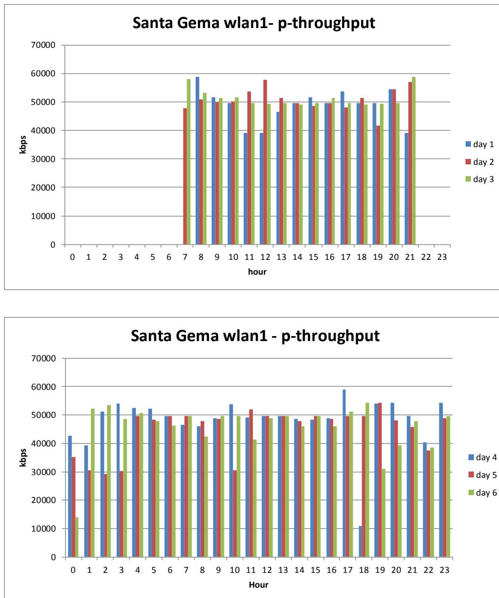
Figure 46: p-throughput measured 3 days before the maintenance and 3 days after the maintenance at the Santa Gema repeater
