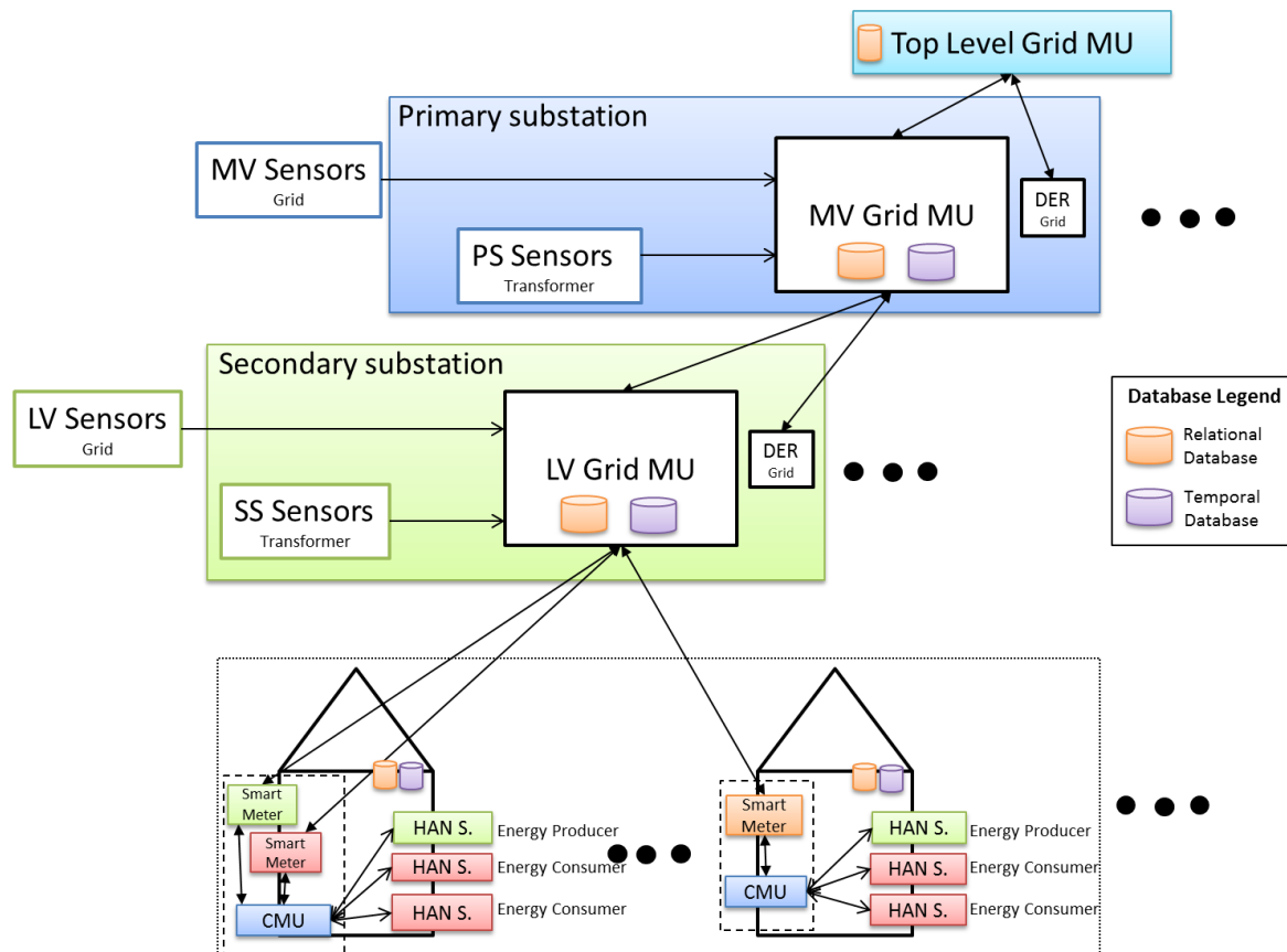
Figure 8: The e-balance data storage architecture
