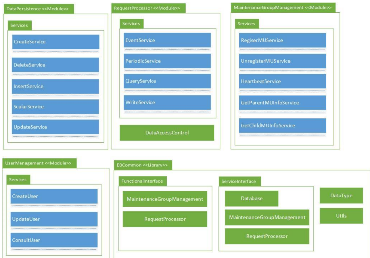
Figure 4 – Package Diagram
