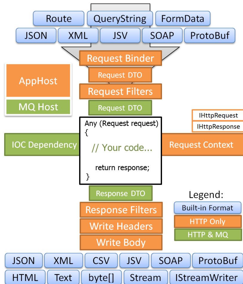
Figure 13 – ServiceStack Server Architecture
