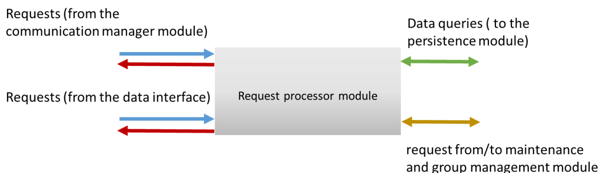
Figure 8 – Request processor module
