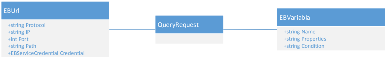
Figure 15 – Query request DTO
