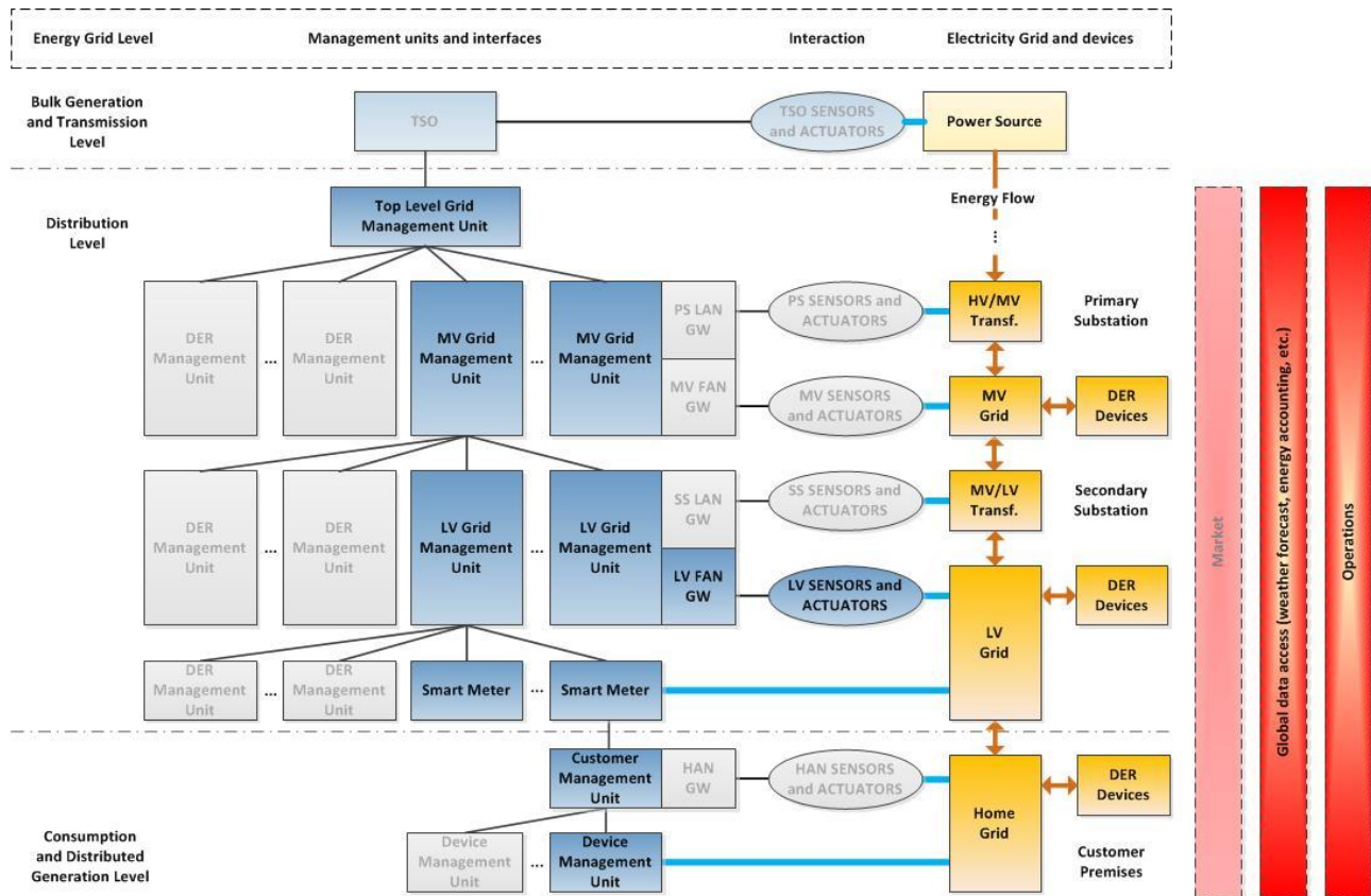
Figure 4: Detailed system architecture for grid resilience serving the Batalha demonstrator
