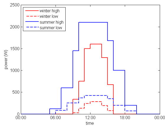
Figure 44: Summer and winter day production profiles
