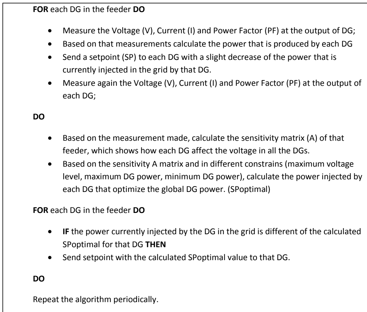
Figure 30: Pseudocode of the voltage control algorithm
