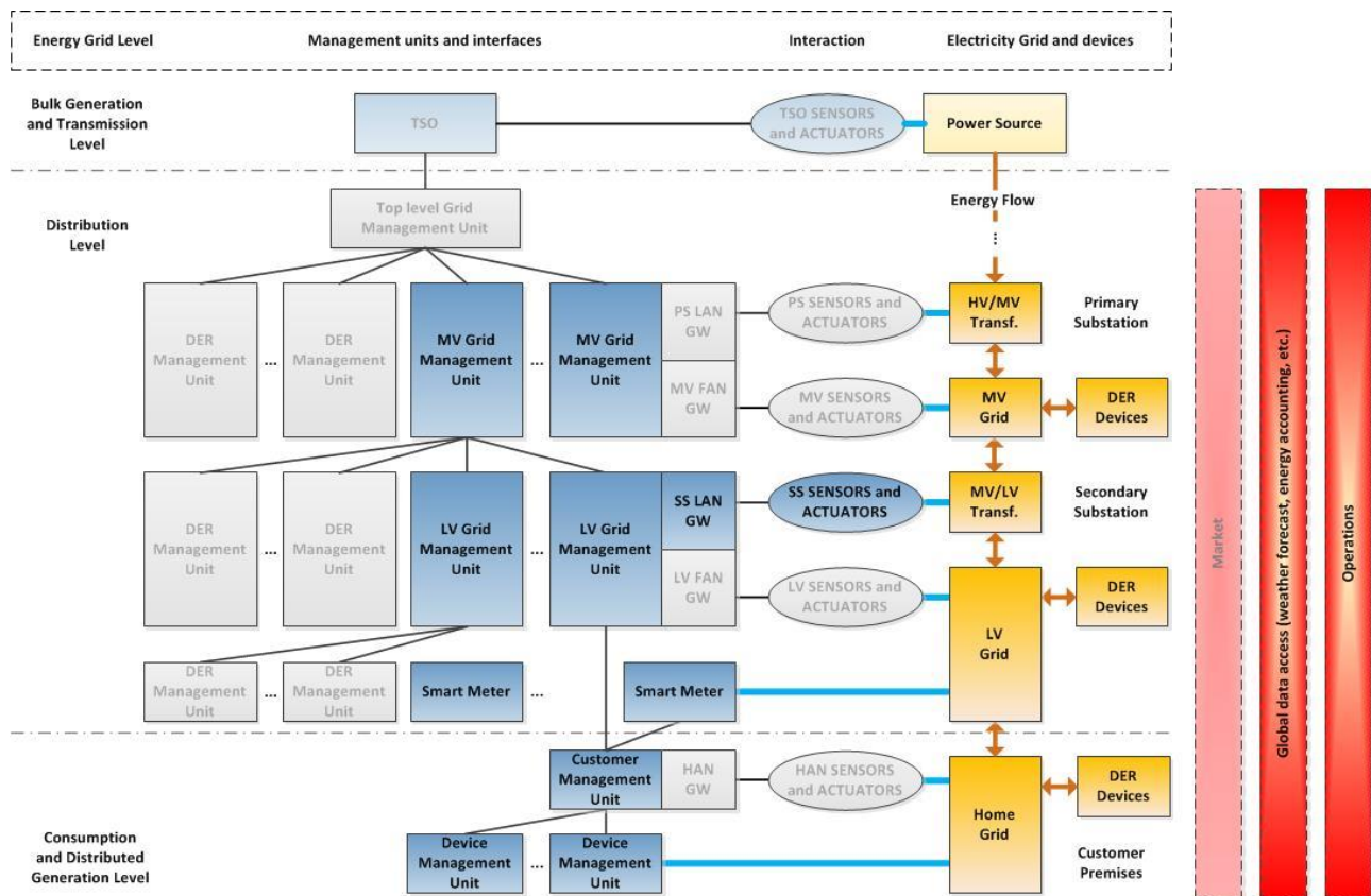
Figure 5: Detailed system architecture for grid resilience serving the Bronsbergen demonstrator
