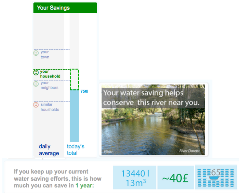
Figure 7. Overview visualizations.
