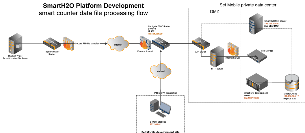
Figure 56. Smarth2O platform development: smart counter data file processing flow.
