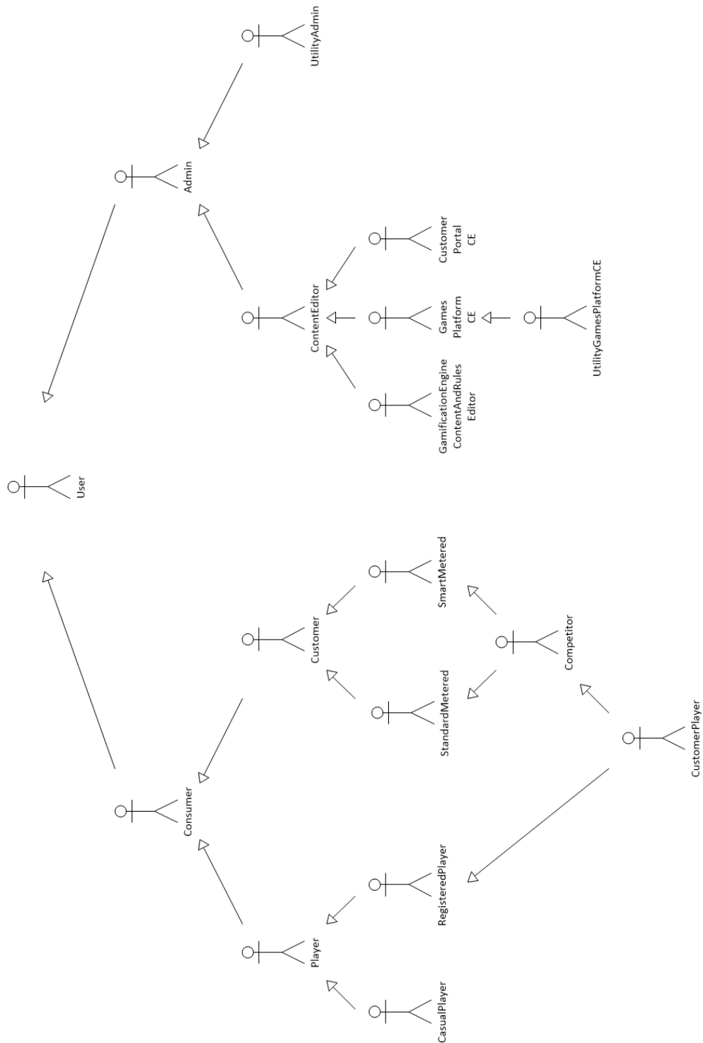
Figure 42. User model.
