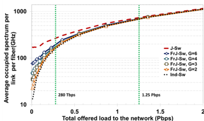
Figure 5: Average occupied spectrum per link per fibre for Ind-Sw, J-Sw and FrJ-Sw (with number of fibres per group (G) varying from 2 to 6) in an SDM network based on bundles of 12 SMFs
