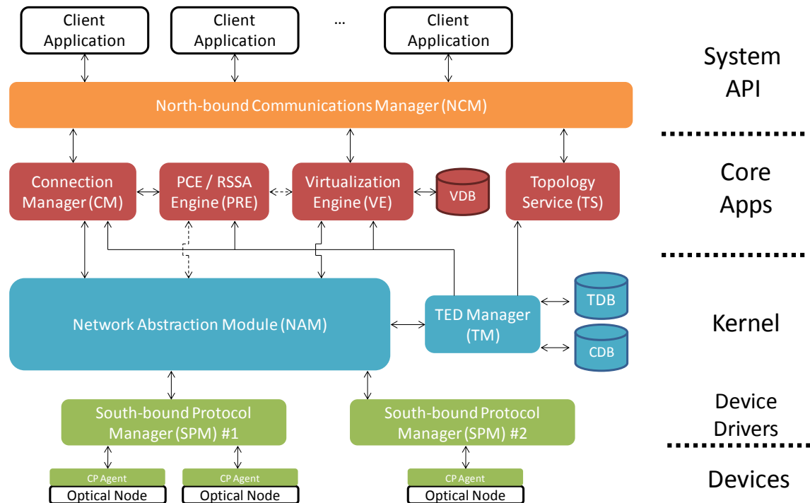
Figure 9 - INSPLACE control architecture (including the most relevant modules and interfaces).
