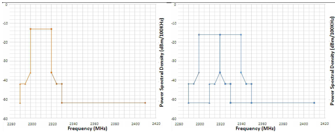
Figure 2.10: Spectrum Emission Mask in Band 40 (20MHz (left) and 40 MHz (right) channel bandwidth) in the femtocell.
