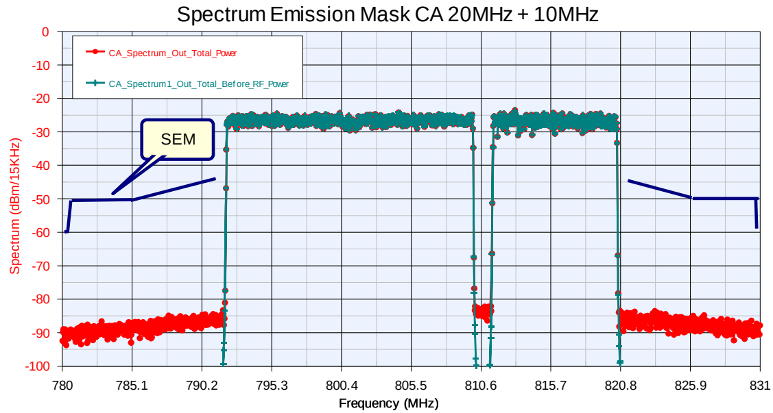
Figure 4.41: Transmitter Spectrum Emission Mask for CA 20MHz+10MHz (red line) and SEM limits (blue line).
