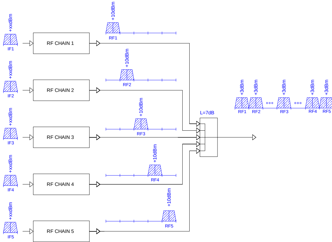
Figure 2.16: Basic architecture of transmitter
