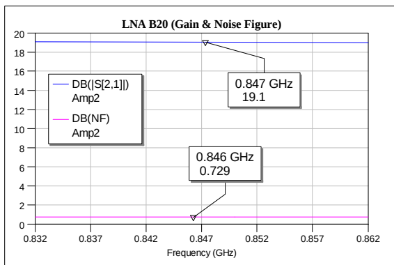
Figure 4.28: B20 LNA main characteristics
