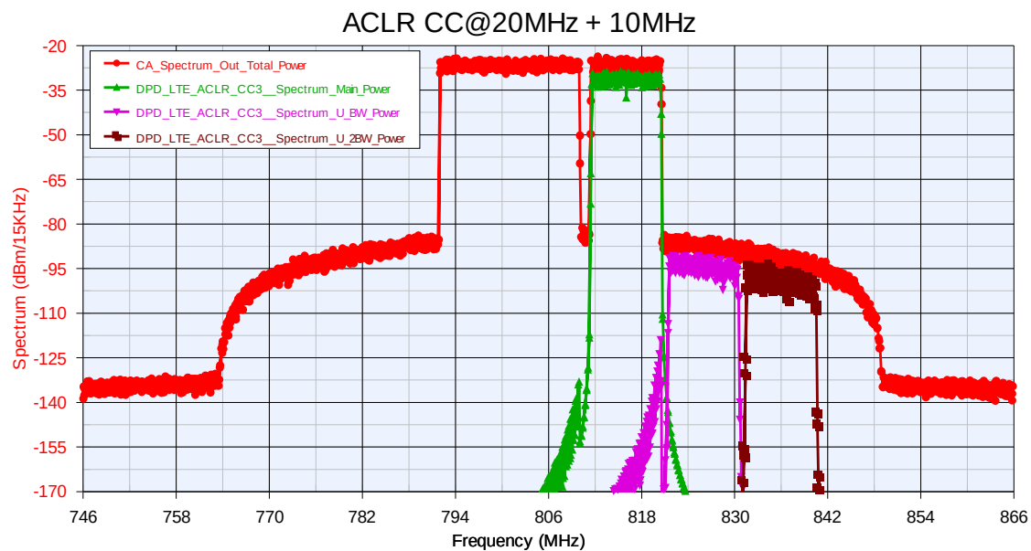
Figure 4.40: Filtered 10MHz adjacent channels for ACLR measurement with RF impairments
