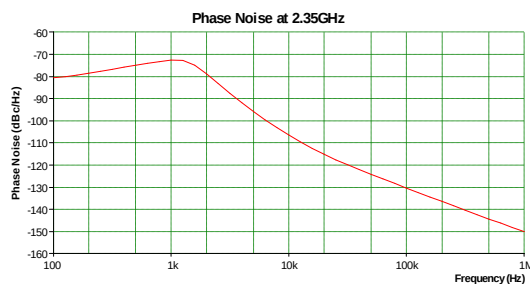
Figure 4.9: LO phase noise (at 2.35GHz)
