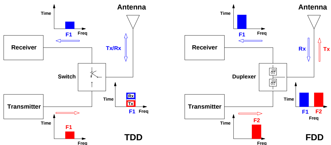
Figure 3.1: Architecture for TDD and FDD
