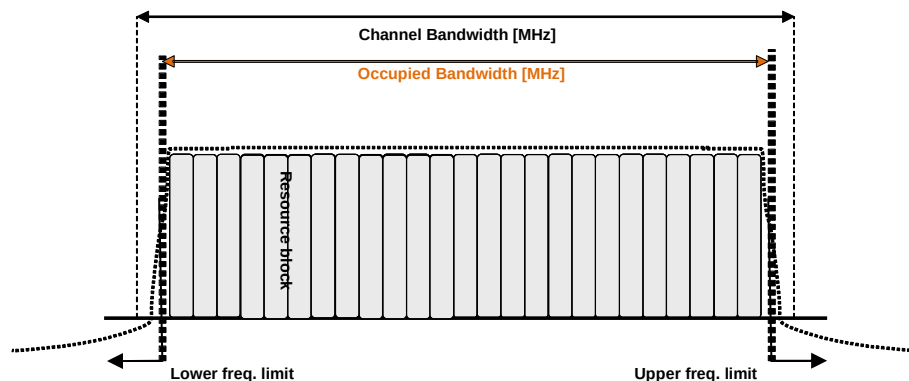
Figure 2.2: Occupied Bandwidth
