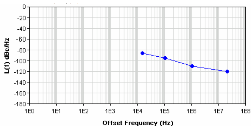
Figure 2.21: Phase noise L(f) (maximum limits) in dBc/Hz for 1^\circ\text{rms} between 15 KHz and 20 MHz
