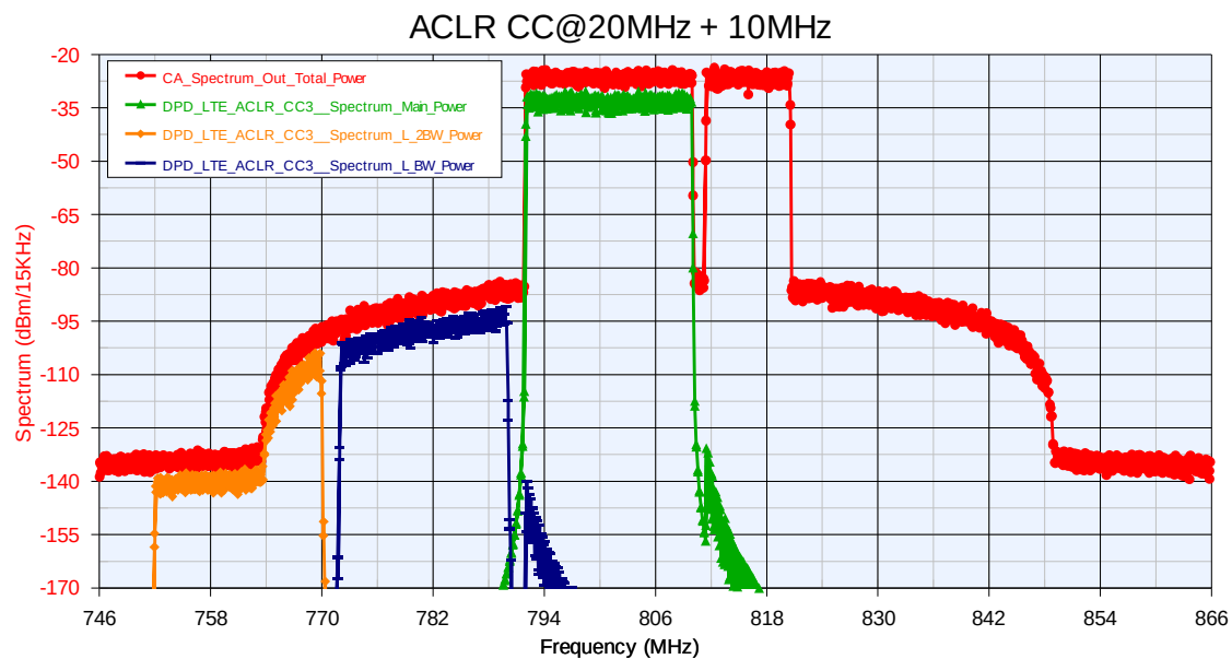
Figure 4.38: Filtered 20MHz adjacent channels for ACLR measurement with RF impairments
