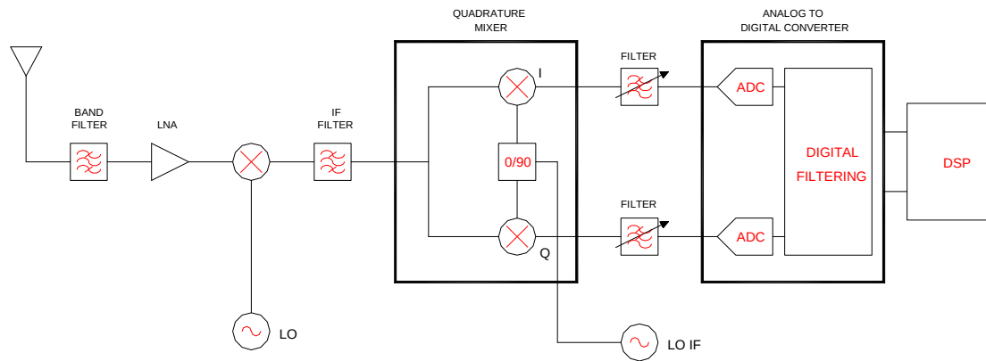
Figure 3.2: Superheterodyne receiver
