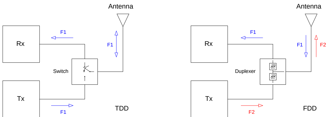
Figure 2.15: Basic architecture scheme for TDD and FDD
