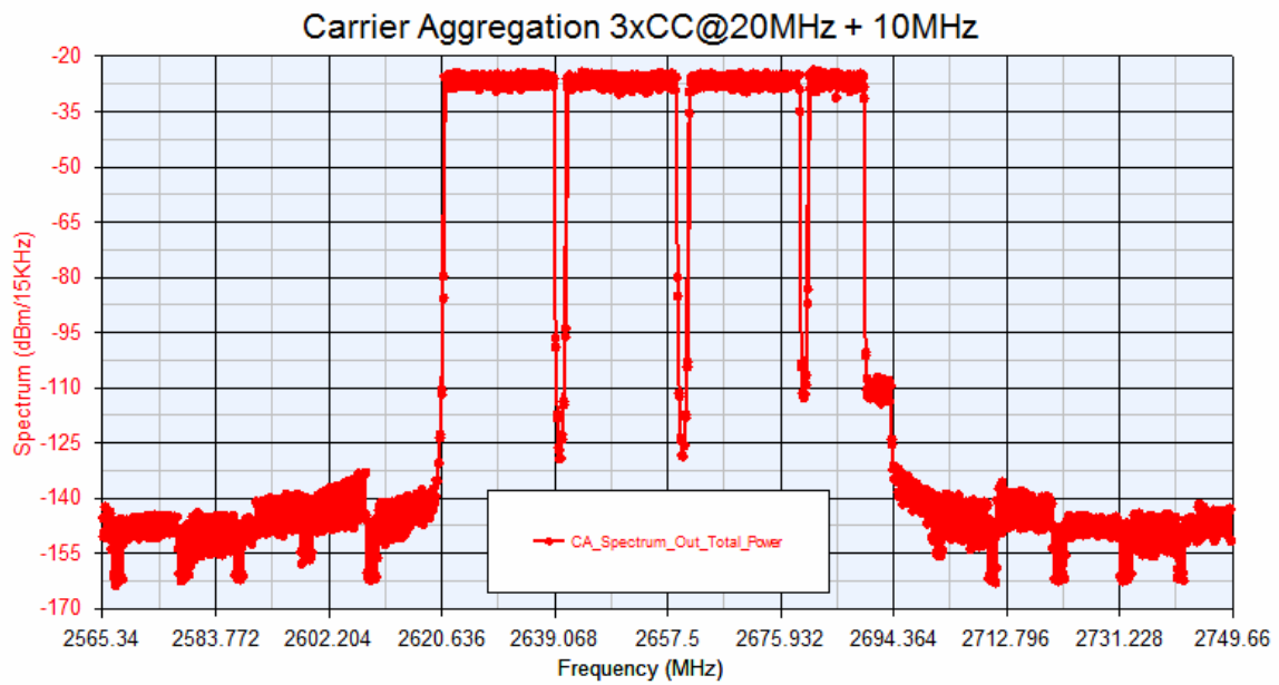
Figure 4.45: Output Spectrum 3xCC@20MHz + 1CC@10MHz Contiguous Carrier Aggregation with NO RF impairments
