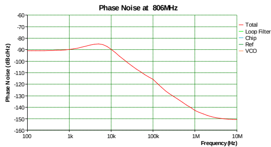
Figure 4.27: LO phase noise (at 806MHz)
