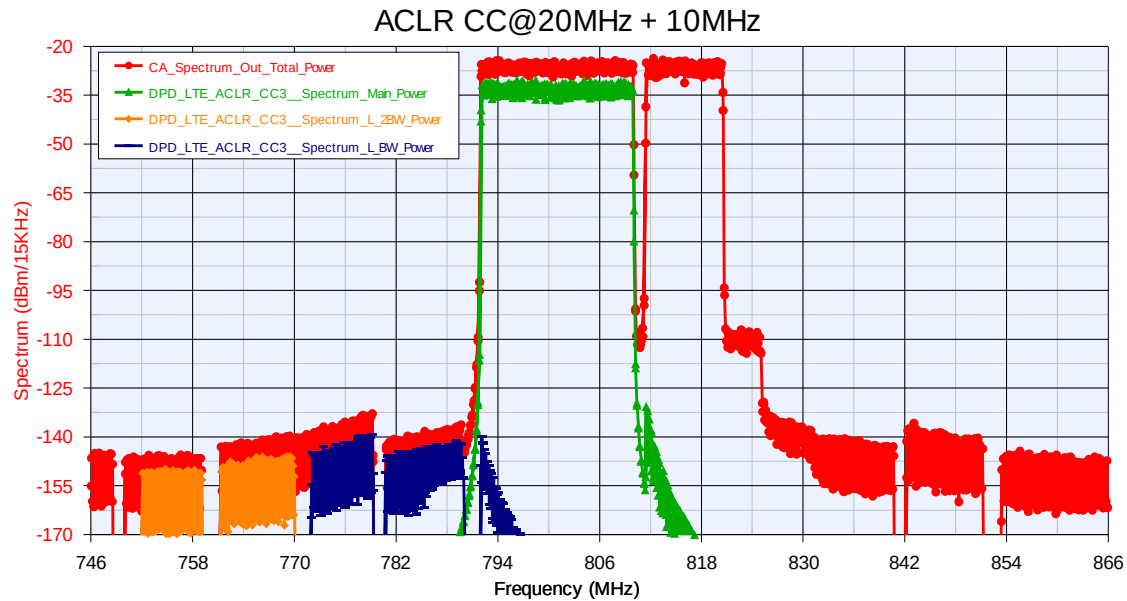
Figure 4.37: Filtered 20MHz adjacent channels for ACLR measurement with no RF impairments
