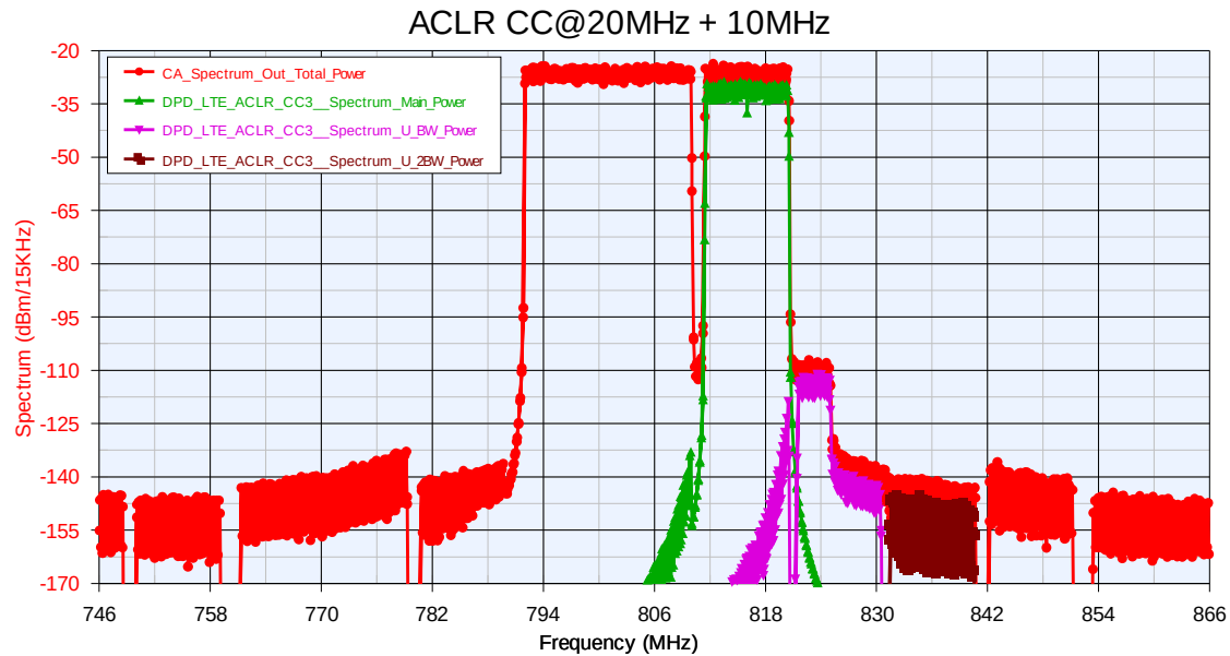
Figure 4.39: Filtered 10MHz adjacent channels for ACLR measurement with no RF impairments
