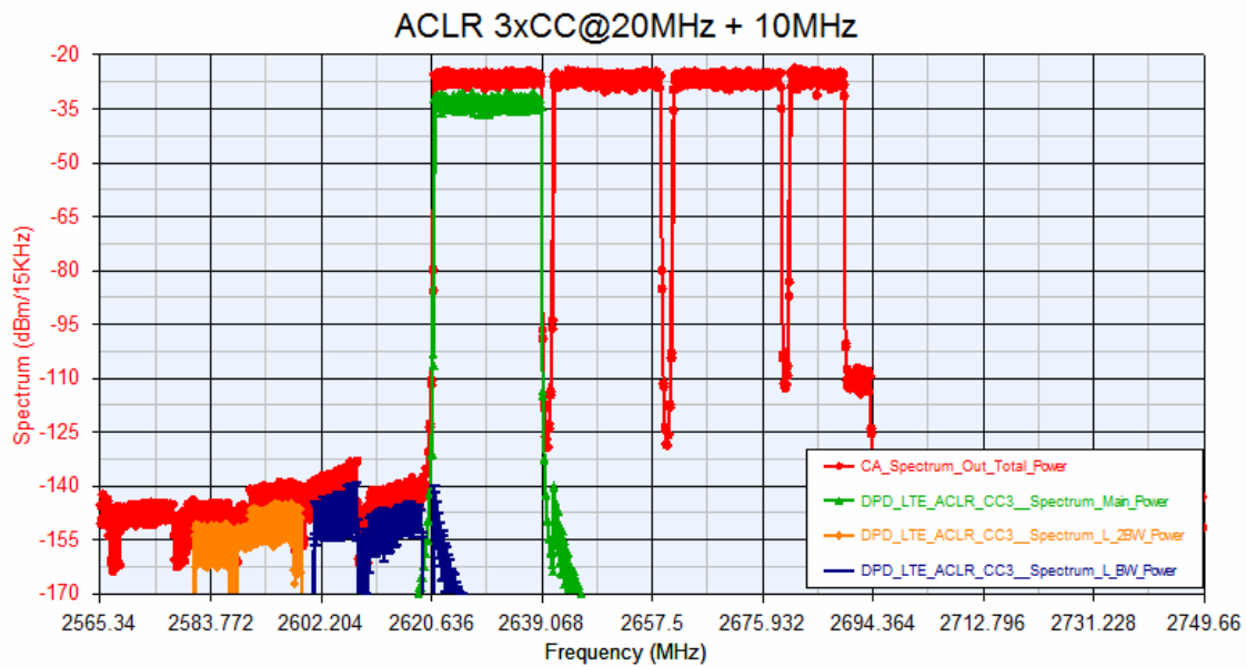
Figure 4.47: Filtered 20MHz adjacent channels for ACLR measurement with no RF impairments
