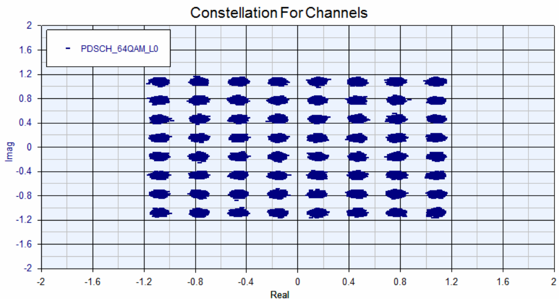
Figure 4.54: Constellation for PDSCH 64QAM channel, with RF impairments
