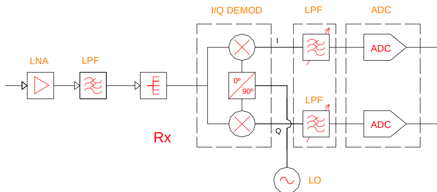
Figure 2.19: Basic architecture of individual receiver chain
