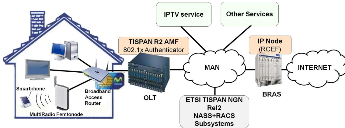
Figure 4-1: Testbed 3 architecture
