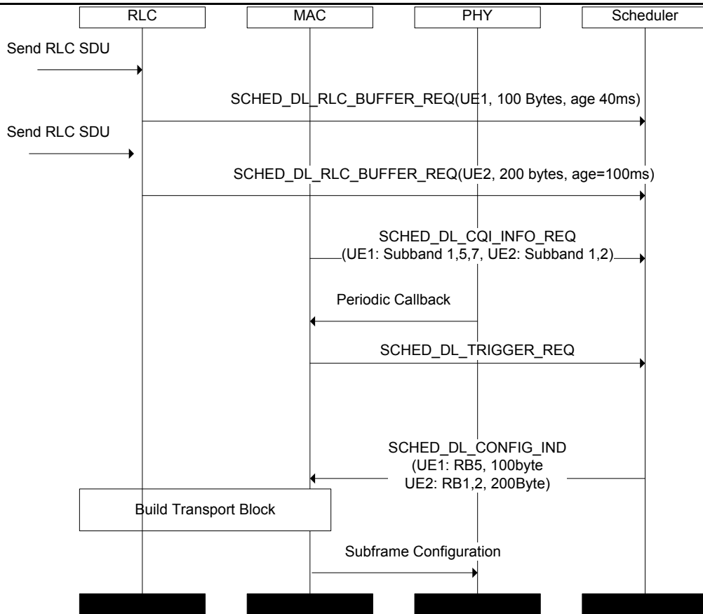
Figure 2-16: Downlink scheduling
