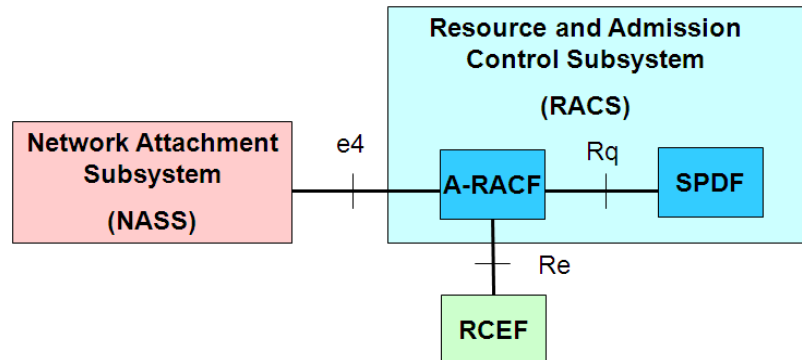
Figure 4-4: RACS architecture
