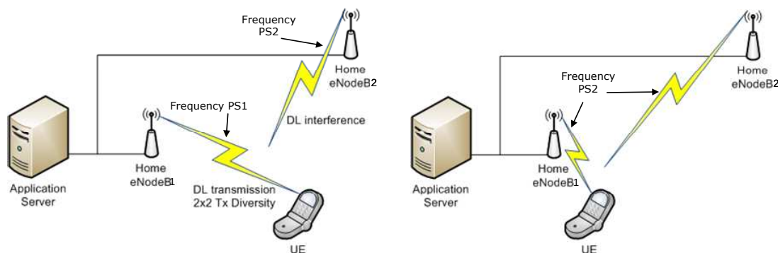
Figure 2-3 FUE served by HeNB1 moves from cell edge (left), to cell centre (right)
