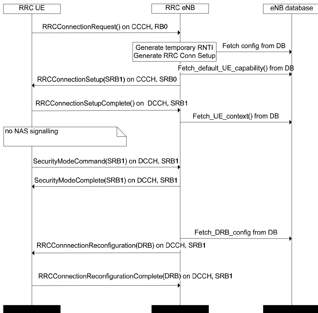
Figure 2-14: Signalling flow
