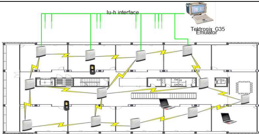
Figure 3-2: 12-node network of femtocells
