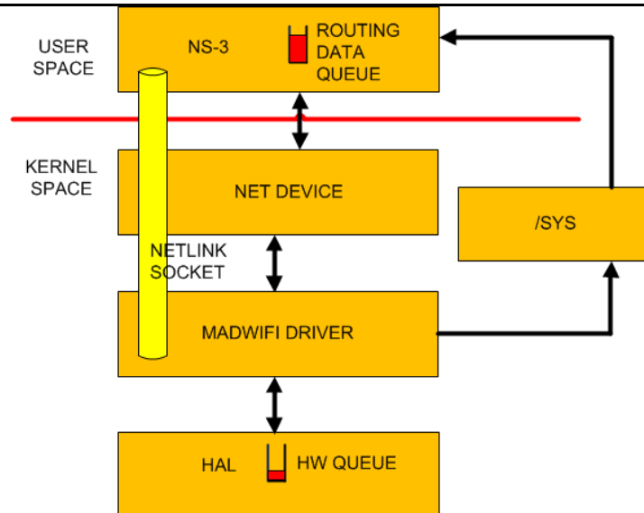
Figure 3-4: User/kernel interaction through the /sys subsystem
