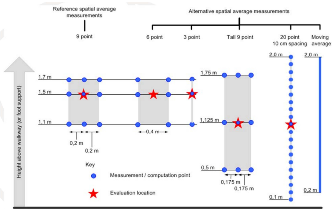
Figure 1: Measurements grids for spatial averaging in IEC 62232.
