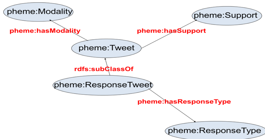
Figure 9: the properties of the ResponseTweet class
