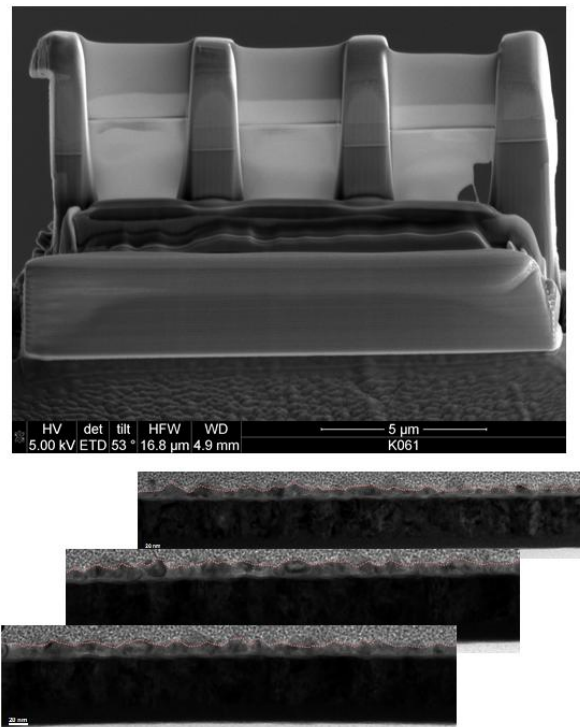
Figure 12: Roughness monitoring
