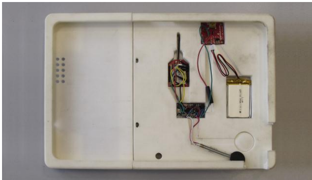
Figure 7. First prototype
