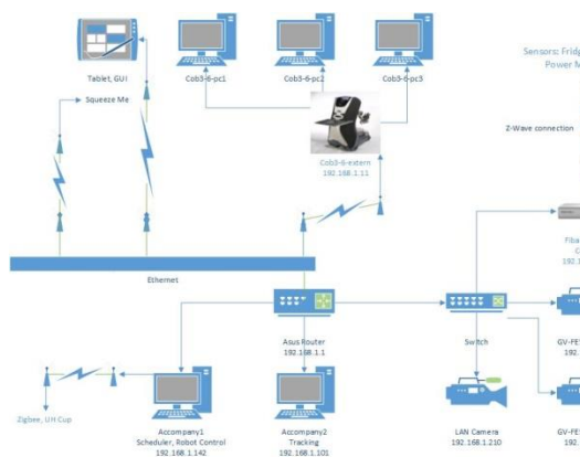
Figure 18 Network map of connected hardware of the ACCOMPANY system.
