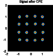
Resulting 16QAM constellation at 3GHz at first driver stage output
