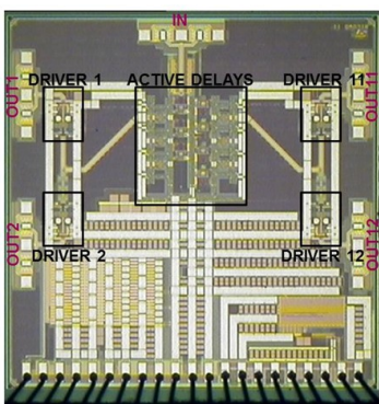
Photomicrograph of the driver testchip
