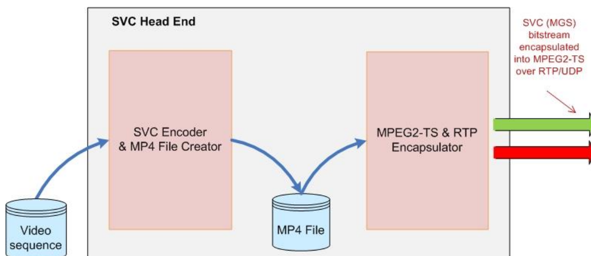
Figure 20 – SVC Head End
