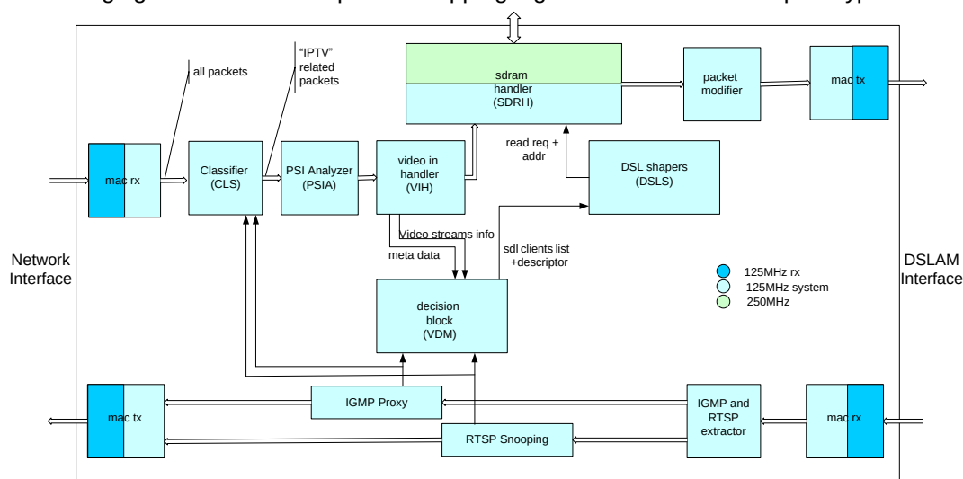
Figure 2 - PDA Top level block diagram
