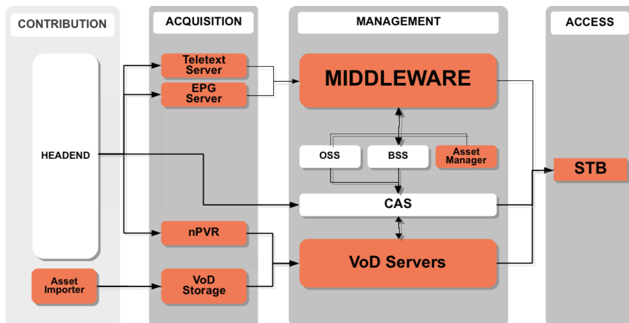
Figure 7 - Middleware deployment
