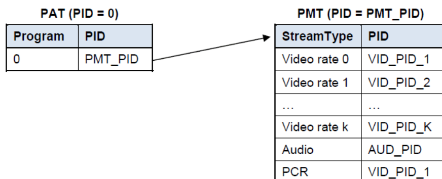
Figure 10 - MPEG-2 transport stream Program Specific Information
