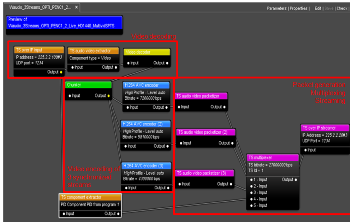
Figure 13: Multi-video-Encoders workflow
