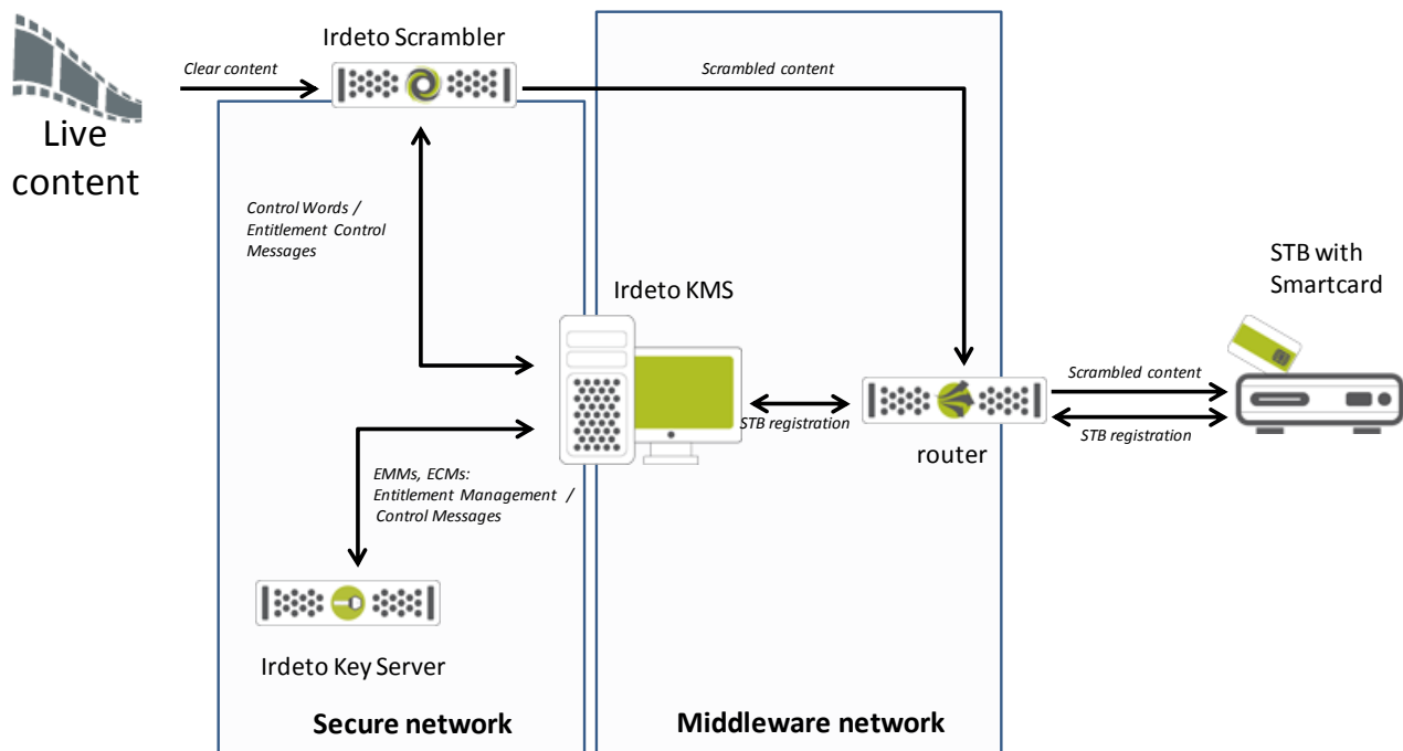
Figure 22: Description of the encryption configuration for the STB-based descrambling
