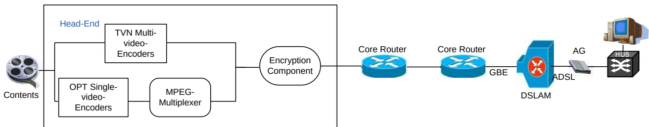
Figure 20: Encryption component installation for the multi-rate approach
