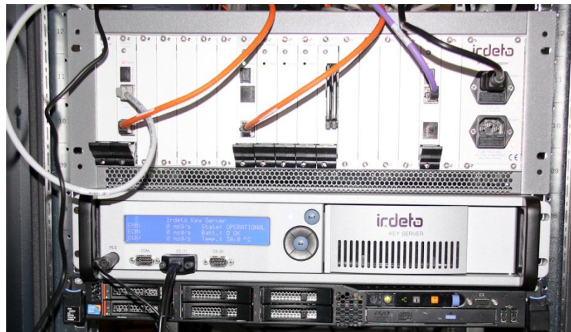
Figure 14: Encryption components: IRD IPTV Scrambler, IRD KeyServer, and IRD KMS
