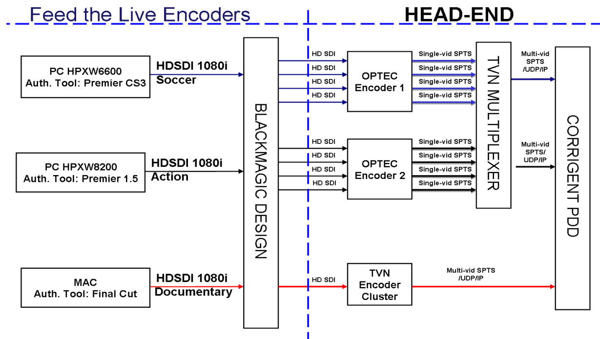
Figure 8: Set-up for Live1/3
