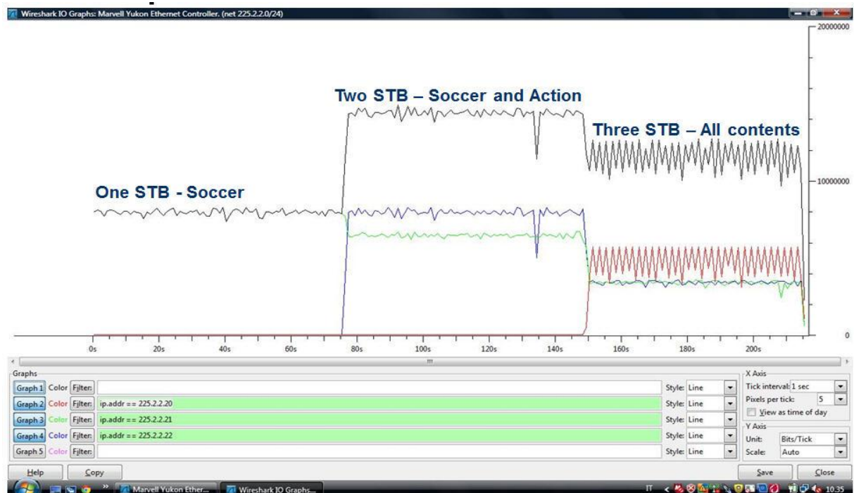
Figure 11: Wireshark acquisition of the used bandwidth by the 3 TV-SETs
