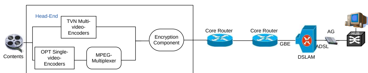
Figure 13: Encryption component installation for the multi-rate approach
