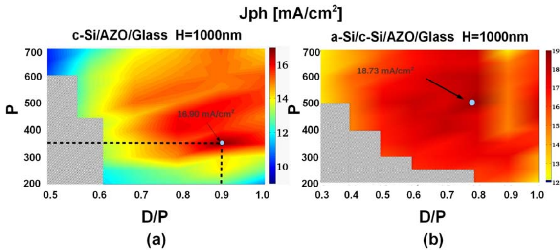
Figure 7 Photo-generated current density maps for (a) c-Si/AZO/Glass nanowires array and for (b) a-Si/c-Si/AZO/Glass core-shell featuring height H=1000\text{nm} . In the former case the optimum geometrical configuration ( P=350\text{nm} , D/P=0.9 ) leads to J_{ph}=16.90
