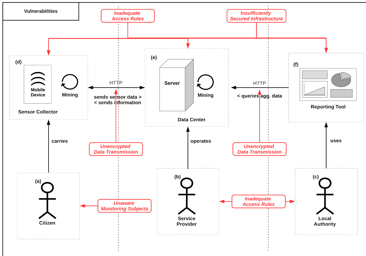
Figure 7: Live+Gov Vulnerabilities
