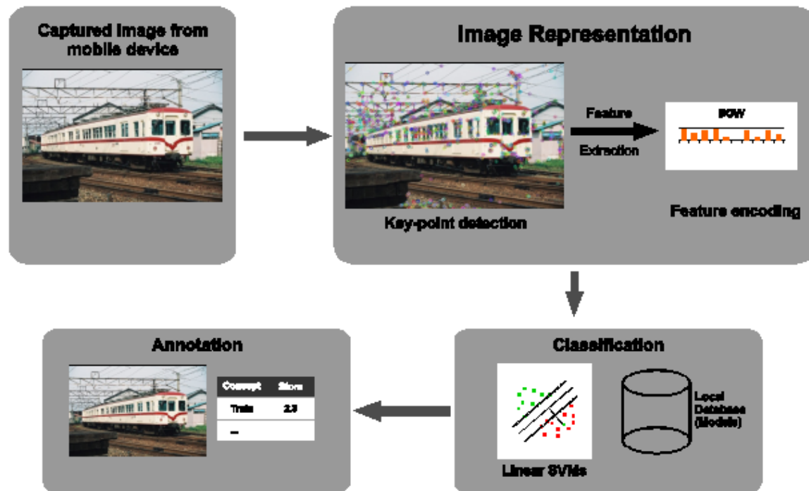
Figure 2: Framework overview for visual recognition
