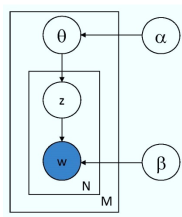
Figure 3: A graphical model explaining the process by which documents are generated.
