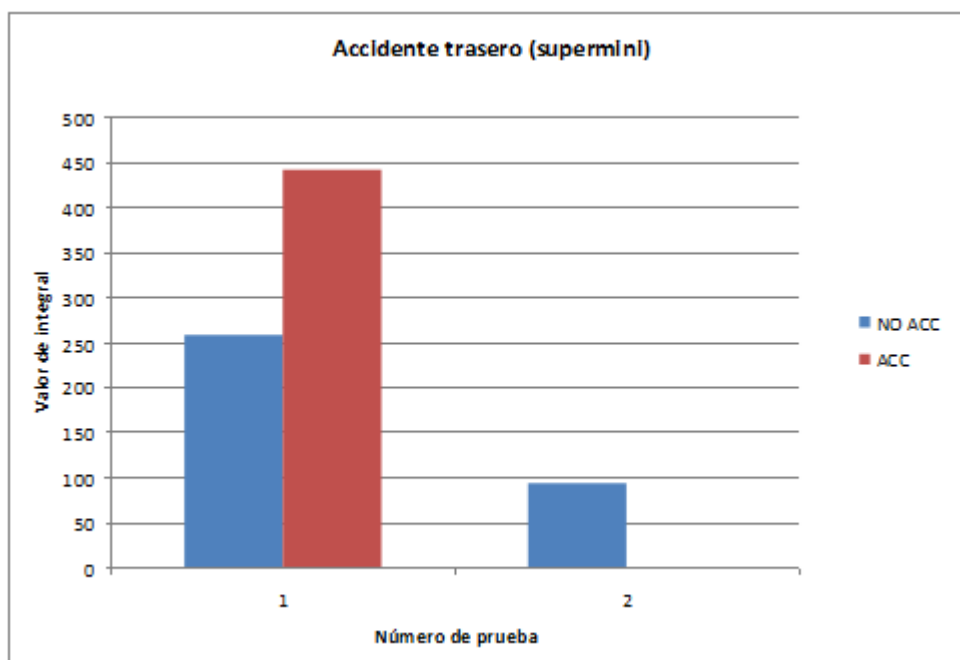
Figure 29: Values of the integral for different rear end accident test in the super-mini class
