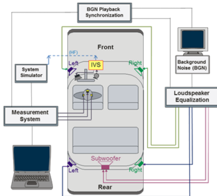
Figure 11: Test arrangement with background noise simulation
