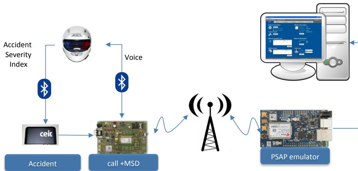
Figure 12: P2W eCall IVS test chain
