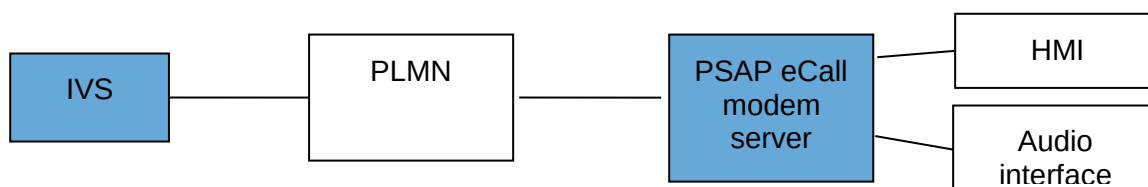
Figure 30: eCall_CFG_01 basic test configuration for interoperability testing
