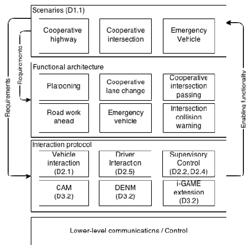
Figure 1 i-GAME functional blocks
