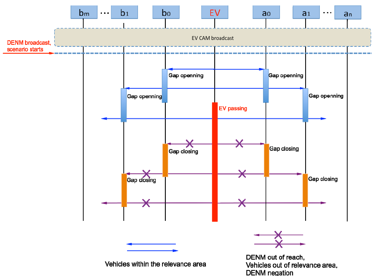
Figure 11 Message flow for the emergency vehicle scenario
