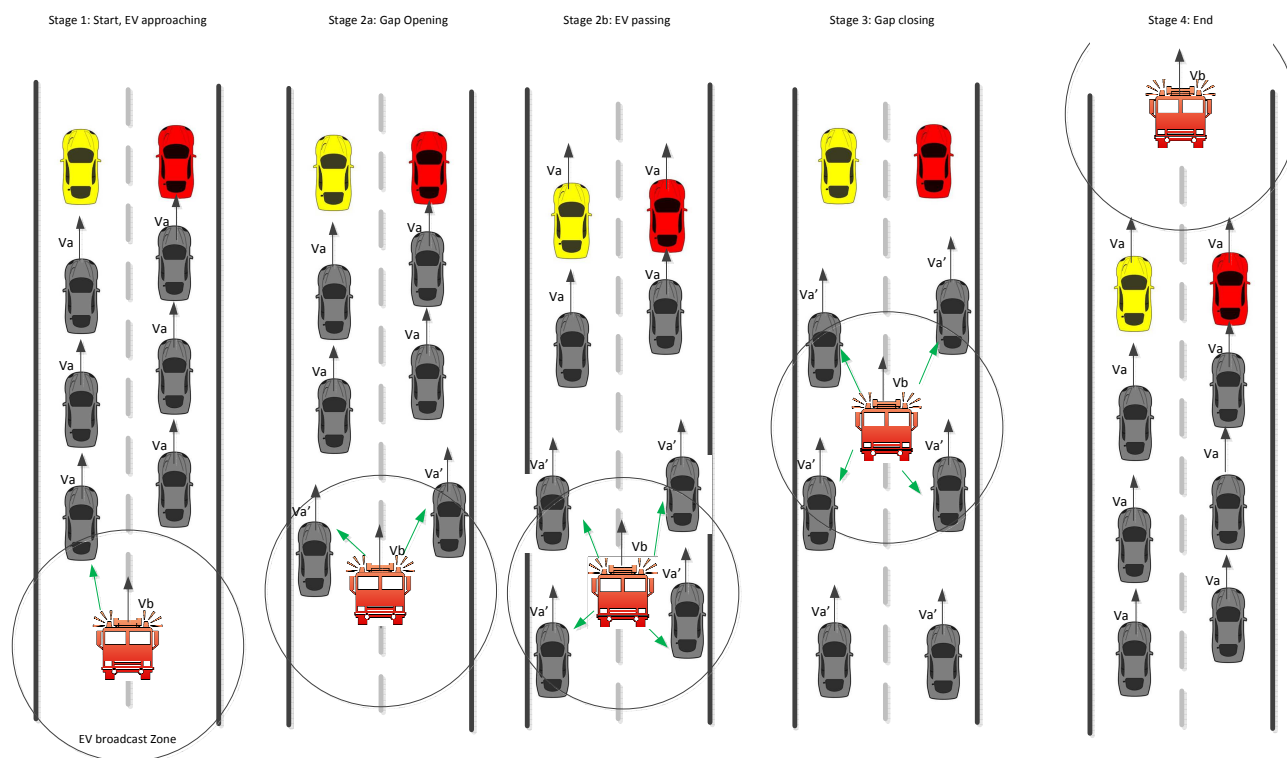
Figure 5 Emergency Vehicle demo scenario
