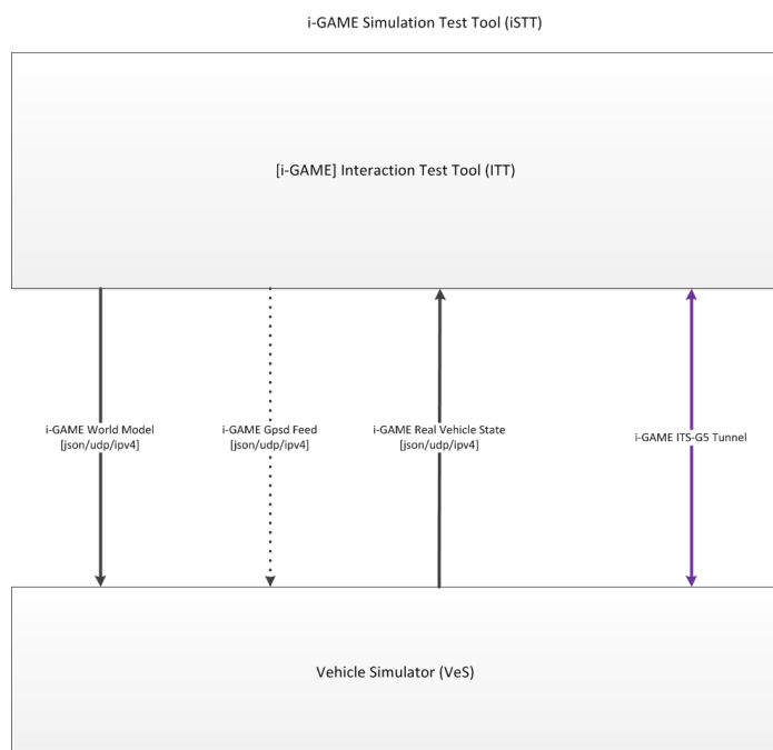
Figure 15: Overview of the i-GAME Simulation Test Tool.
