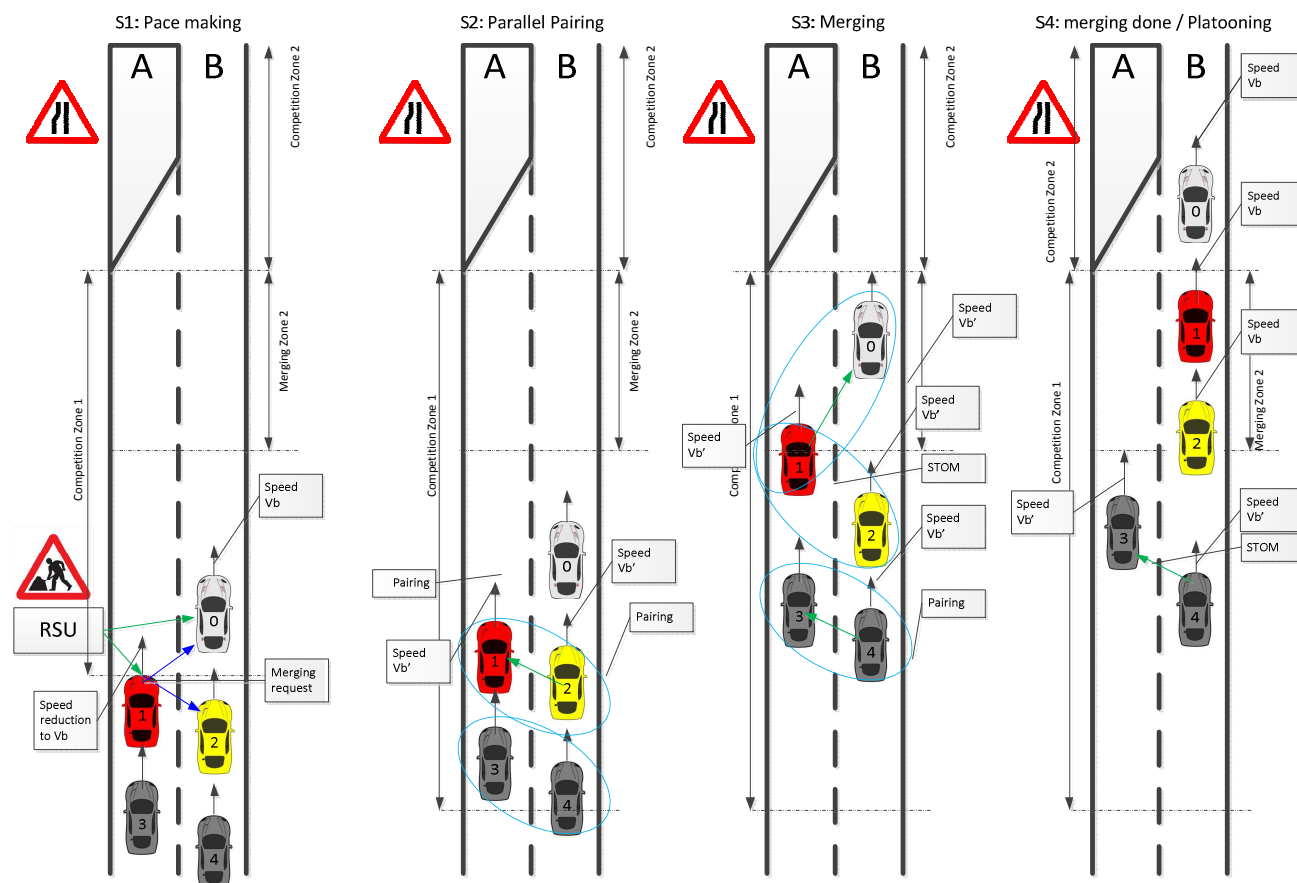
Figure 2 Merging scenario
