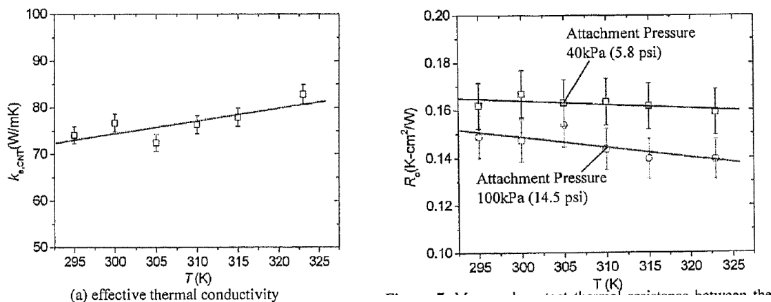
Figure 1 : Effective thermal conductivity (a) and thermal interface resistance (right) of a 13 \mu\text{m} thick CNT film grown on Si by PECVD (from [45])
