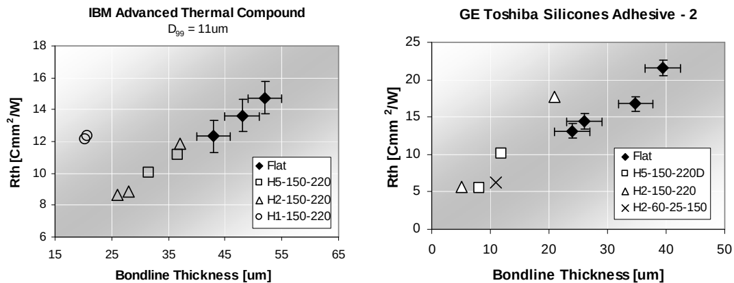
Figure 5 : Thermal resistance benefit from various HNC interfaces compared with a flat surface. (a) IBM ATC D_{99} = 11\mu\text{m} , (b) GE Toshiba Silicones adhesive-2. Bondline conditions: 5 bar assembly load, 19.7-mm-square chip, 200 W, temperature \sim 30^\circ\text{C} .
