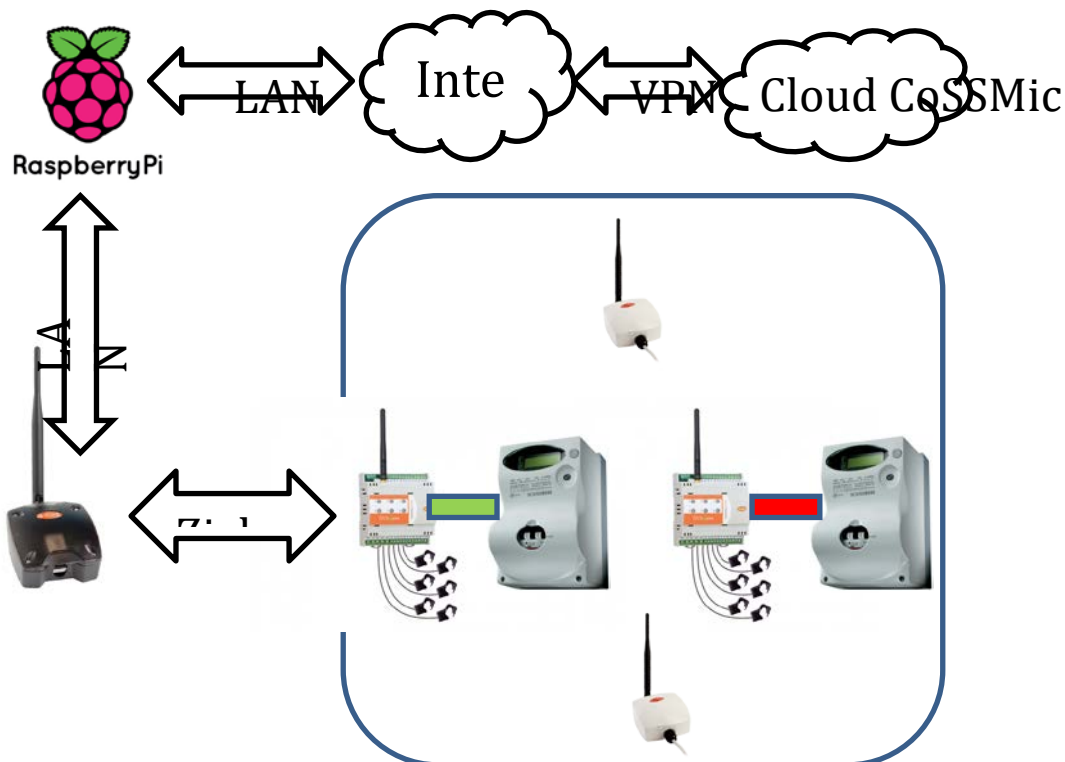
Figure 36: – System Architecture I.T.C Alfonso Gallo - Aversa (CE)
