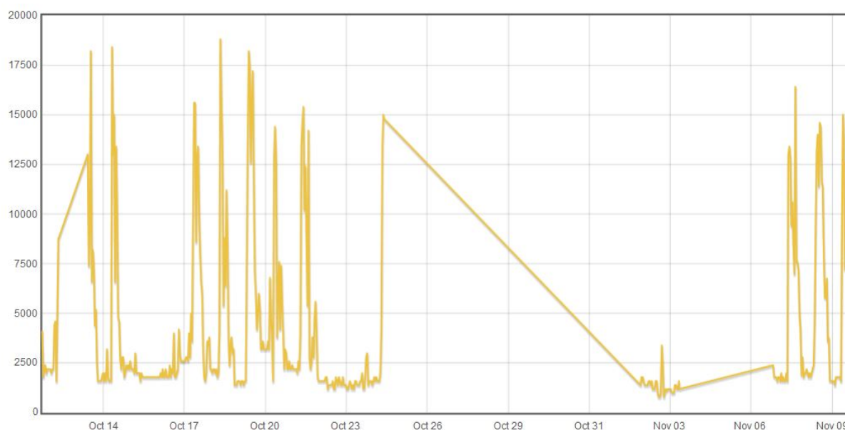
Figure 16: The power consumption of about one month with three longer lasting periods of failure of data transmission.
