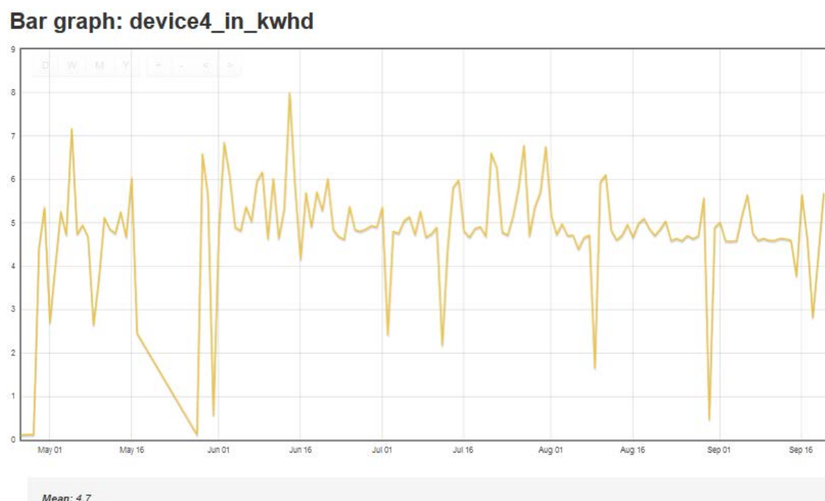
Figure 9: The daily charging in kWh of the stationary battery from May to Sep. 2016. The data loss from 17 th to 28 th May is clearly seen.
