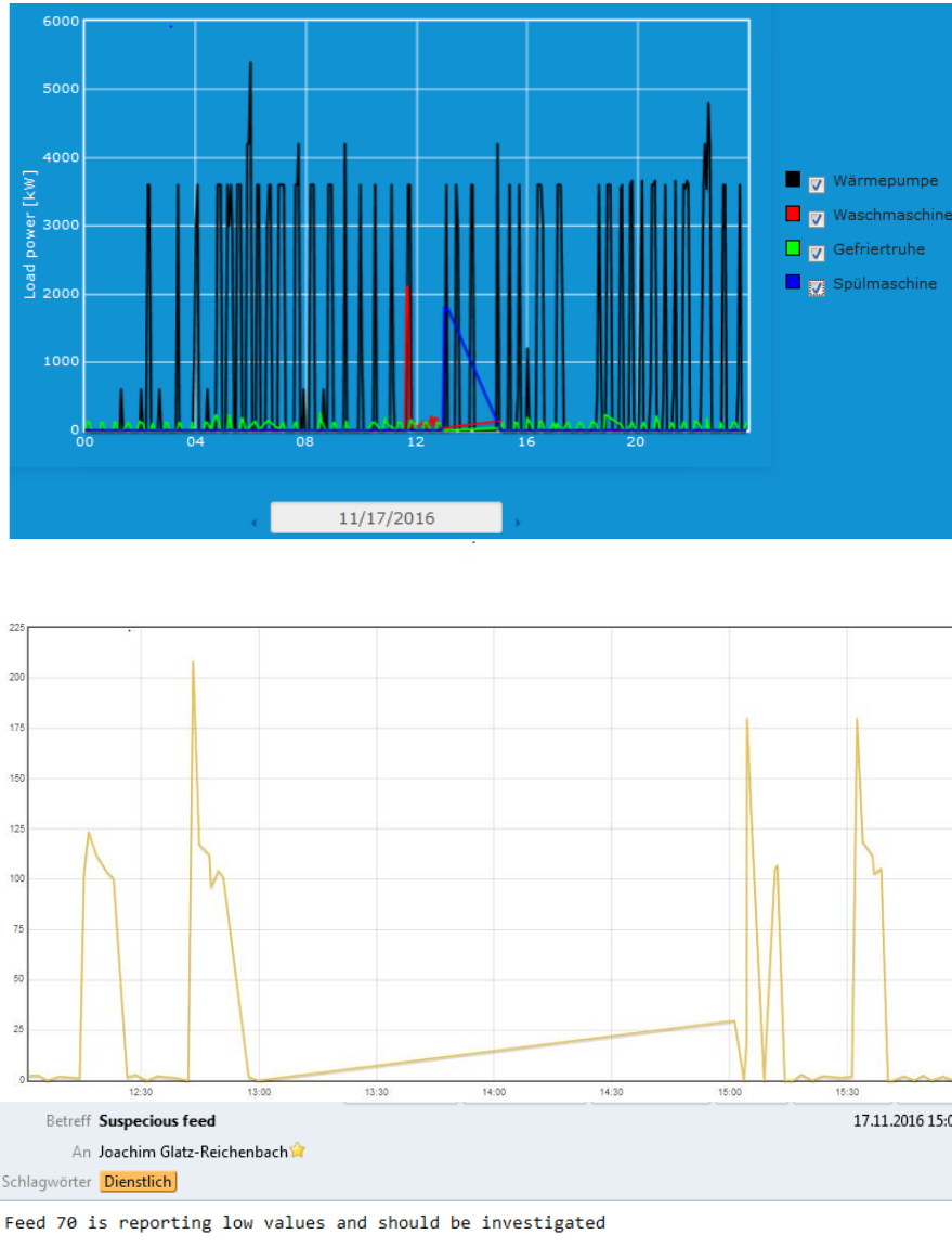
Figure 21: The monitored power consumption of the freezer in the top graph in green together displayed with other monitored appliances, and only the power consumption of the freezer in the middle graph and the sent out alert email message in the bottom part.
