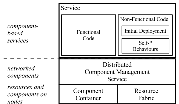
Figure 5: Grid4All Service Programming Framework
