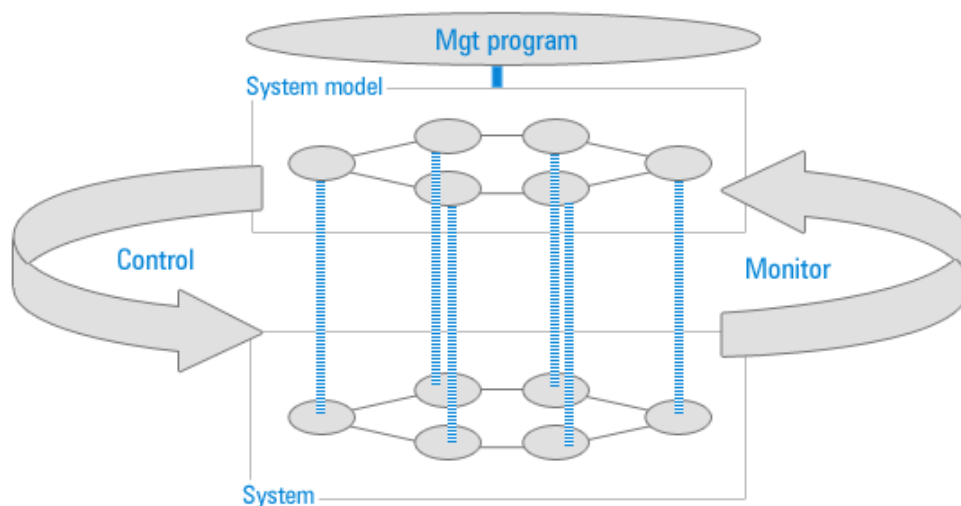
Figure 1: Feedback-based management
