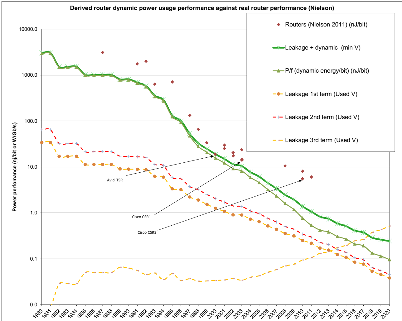
Figure 5-4 Comparison of dynamic VLSI chip power performance and router power performance
