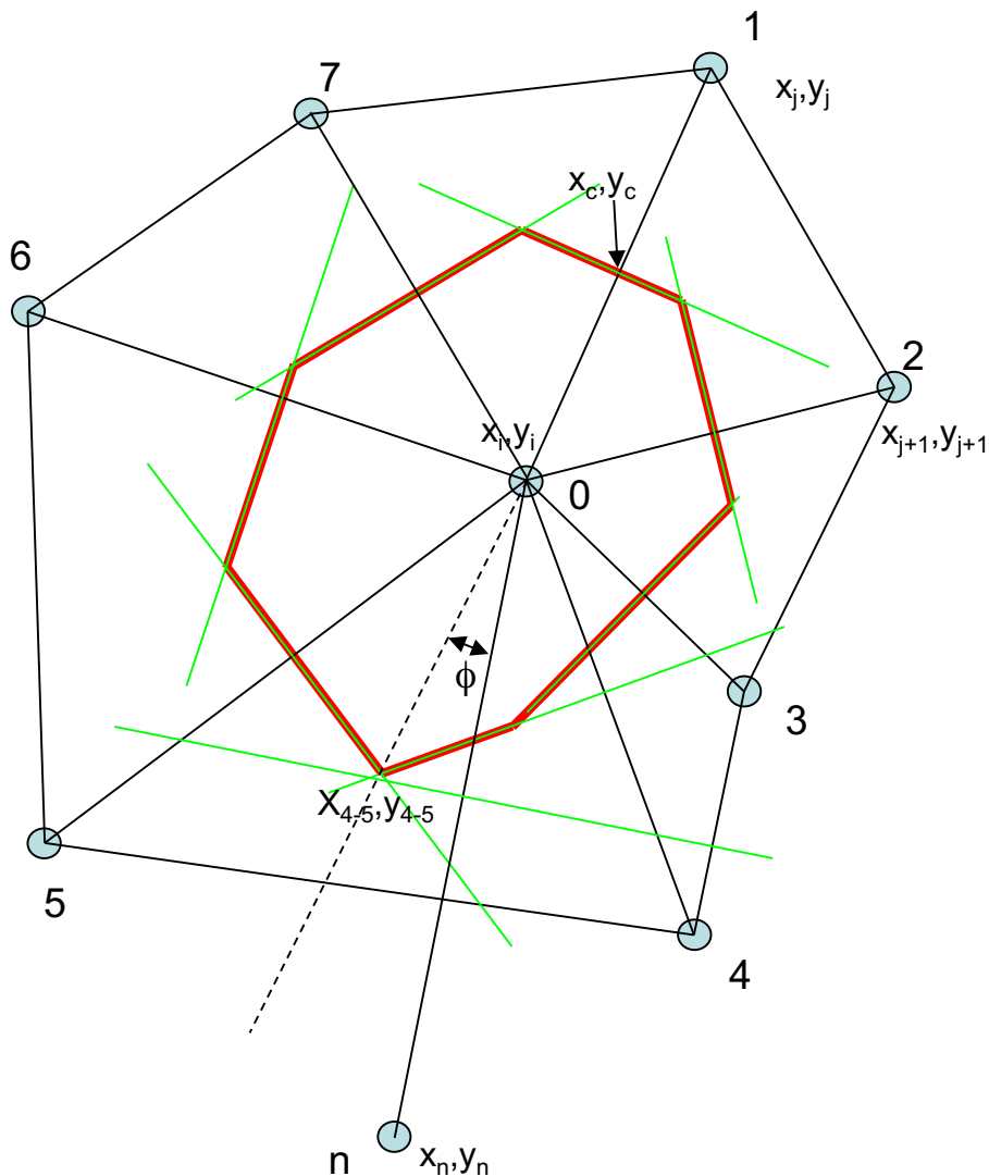
Figure A5-2 The LE at point x_n, y_n lies outside Voronoi polygon
