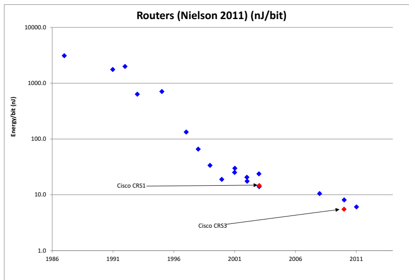
Figure 5-3 Router energy performance (Nielson 2011)
