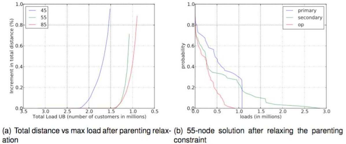
Figure 2-10 Results obtained after the relaxation of the parenting constraint
