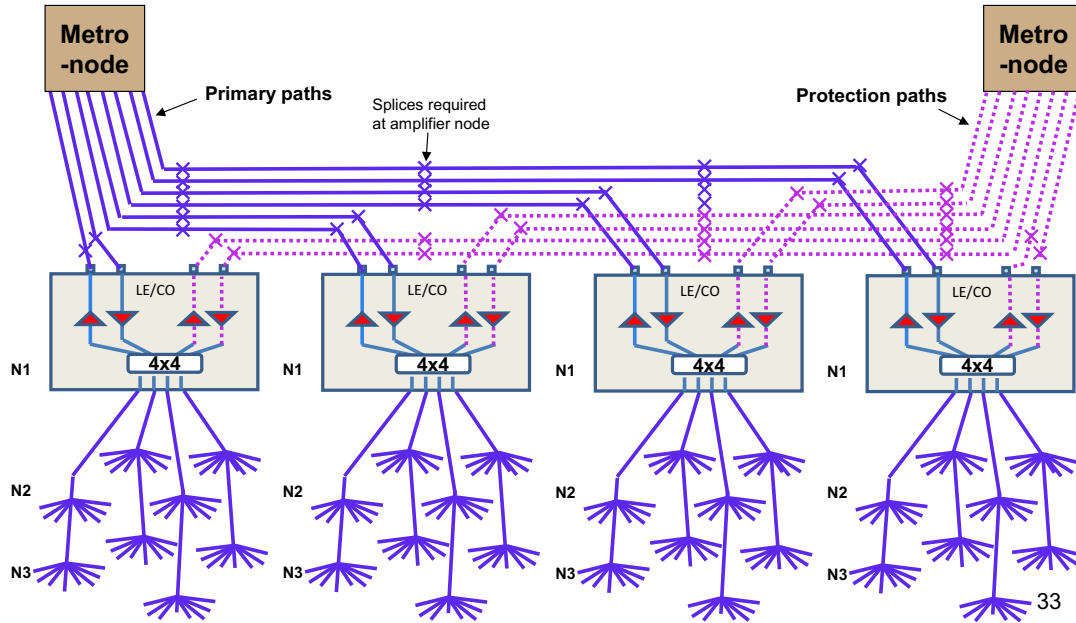
Figure 4-14 Backhaul cable chain model structure
