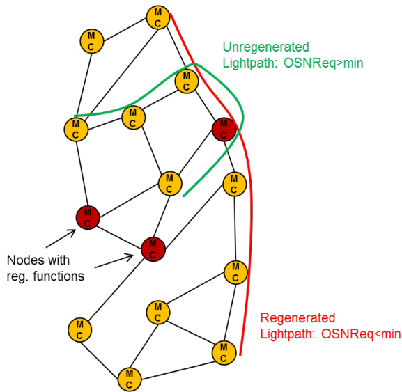
Figure 6-3 Translucent network with sparse regeneration nodes (on the left), and transparent network with sparse Raman amplified links (on the right). In the latter network regenerators are replaced by Raman amplified links thus obtaining a fully transparent network
