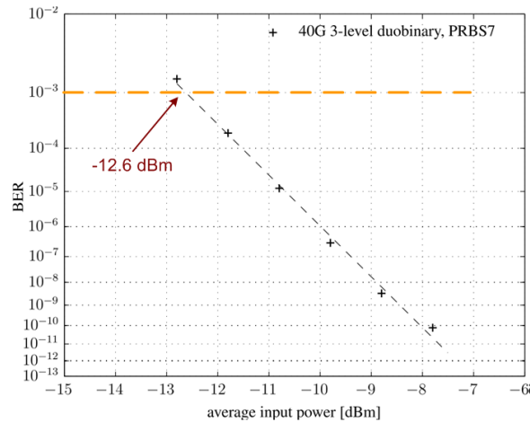
Figure 4-23 measured BER of the 40 Gb/s 3-level duo-binary downstream with PIN-Rx
