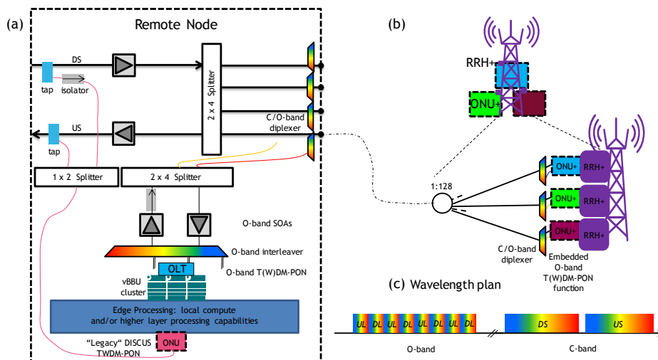
Figure 4-19 Detailed architecture of Figure 4-18 to realize very low latency midhaul link. The remote node configuration is shown in (a), the antenna site is shown in (b) and the wavelength plan to overlay the very low latency links using O-band T(W)DM-PON on top of the legacy DISCUS PON services located in C-band is depicted in (c).
