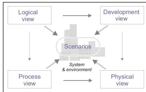
Figure 1: '4+1' architectural view model (Kruchten, 1995)
