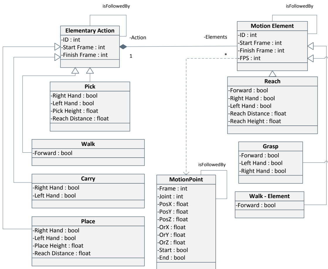
Figure 10: Elementary Actions and Motion Elements model
