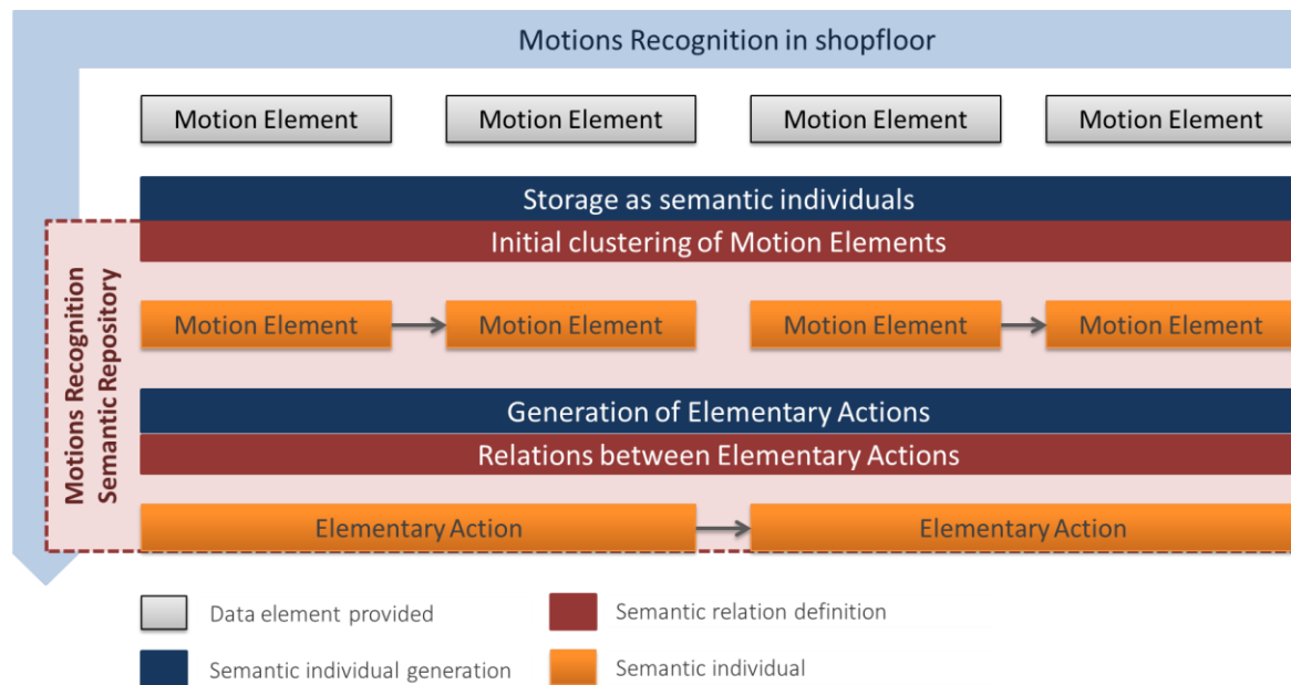
Figure 11: Pipeline of Elementary Actions storage
