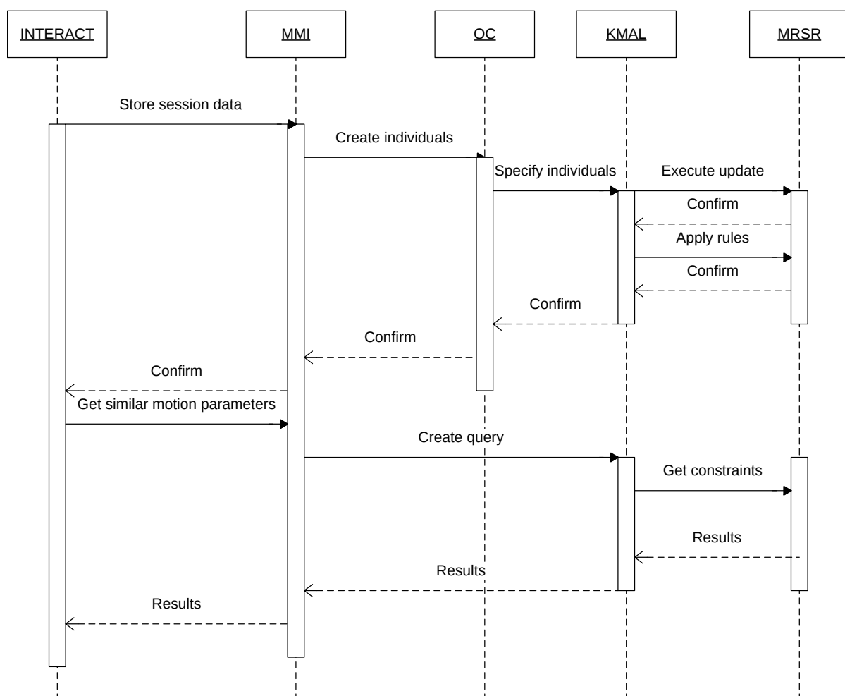
Figure 12: Recognised Motions Management System sequence diagram
