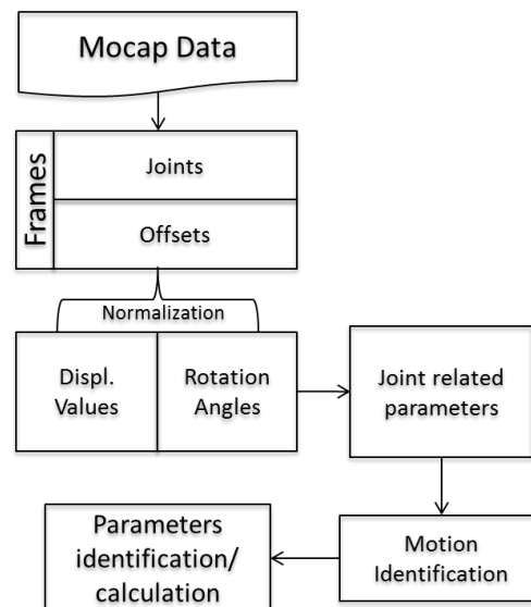
Figure 1: Parameterised Motion Element recognition
