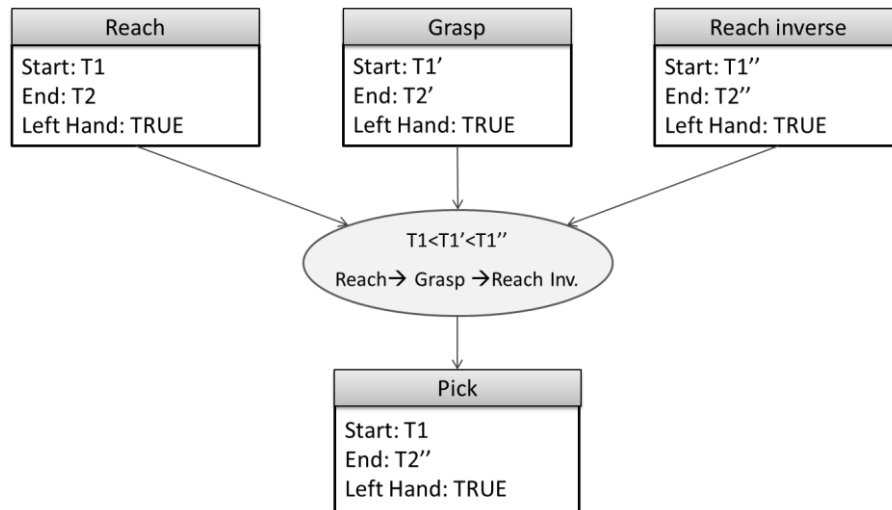
Figure 8: Motion Elements clustering to form a Pick Elementary Action
