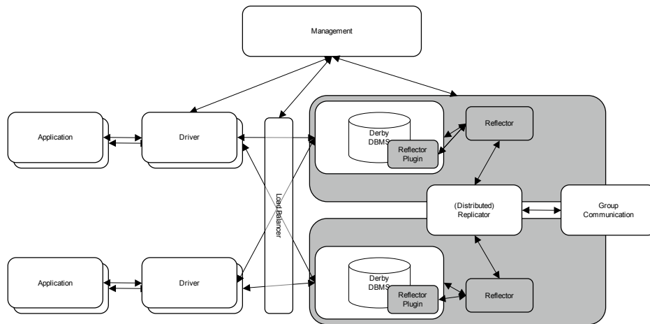
Figure 1.1: Mapping architecture.
