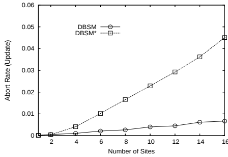
Figure 2: DBSM* vs. DBSM (updates only)
