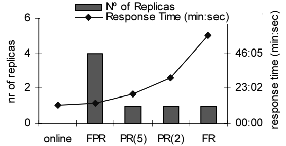
Figure 9: Response Time & Replicas 10 nodes/4 fail (Query 9)
