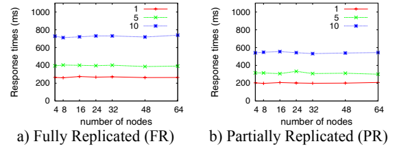
Figure 3. Scale up Results
