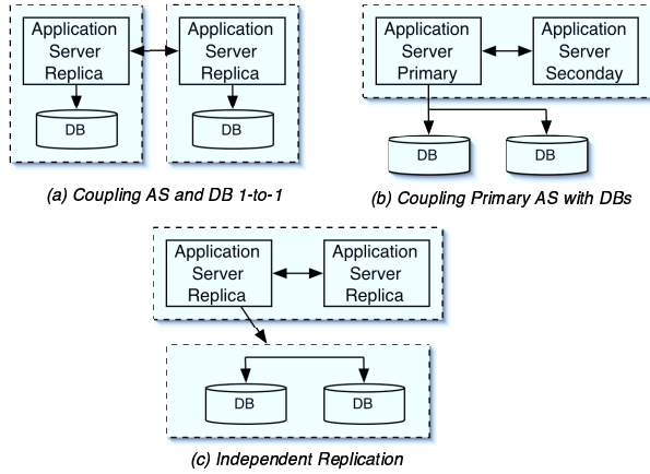
Figure 1: Replication Architectures
