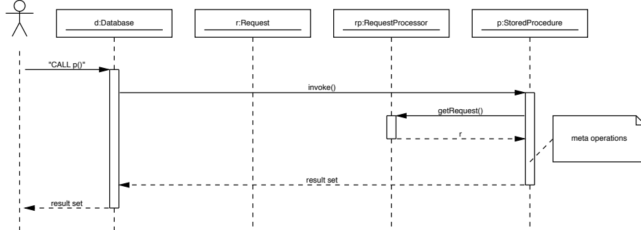
Figure 6: Base-level calls meta-level.
