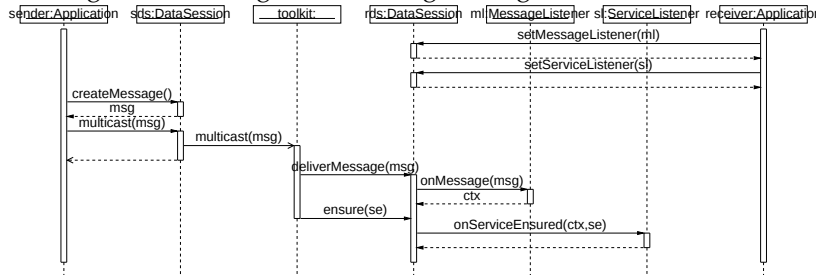
Figure 2: Sending and receiving messages with the services.
