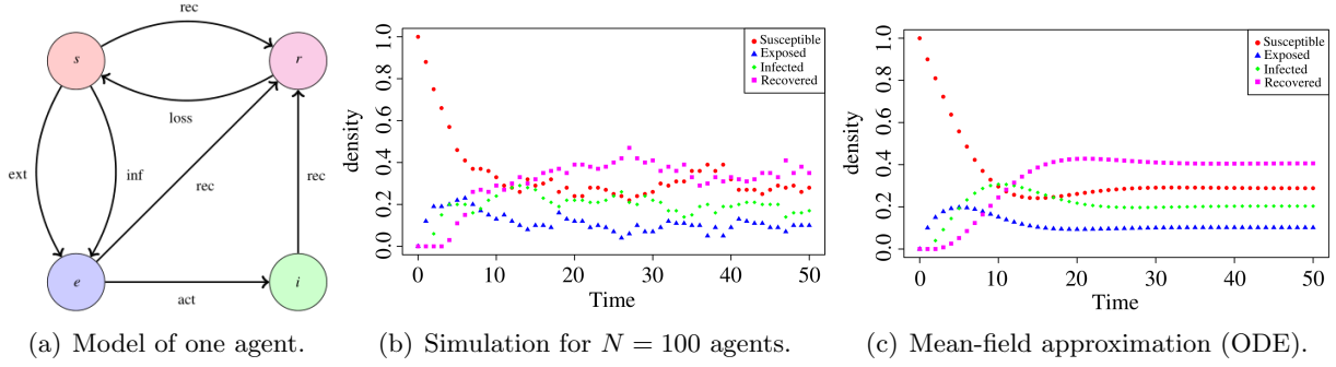
Figure 1: The model of a worm epidemic from [BHL13]. We plot the evolution of the number of agents in each state as a function of time. The behavior of the stochastic system with N = 100 agents is close to the one of the mean-field approximation (courtesy of [BHL13]).
