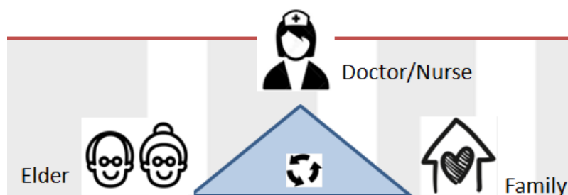
Figure 7: Triangle Communication
