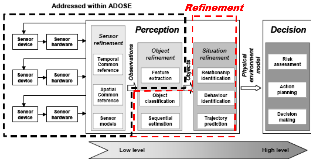
Figure 2: Refinement phase
