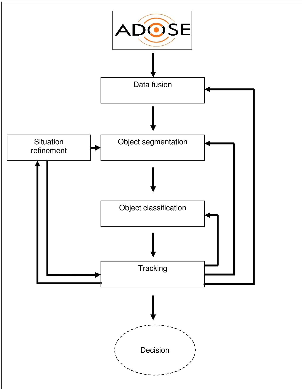
Figure 3: Software - High level
