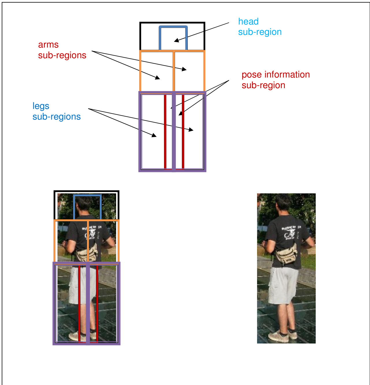
Figure 8: Feature extraction – Pedestrian case example
