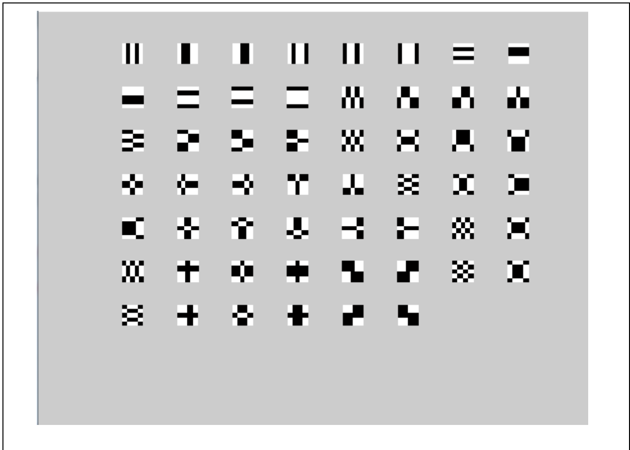
Figure 12: Haar feature
