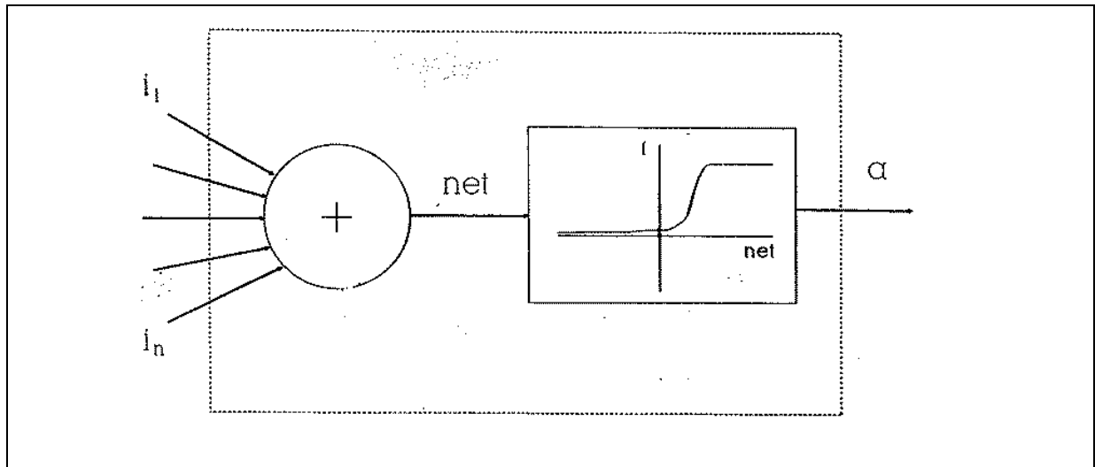
Figure 11: Neuron representation
